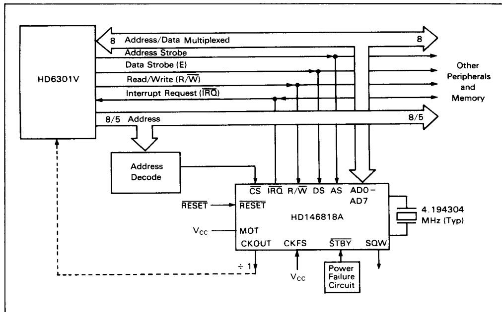
Figure 16. HD146818A Interface with 6301 Family Microcomputers
