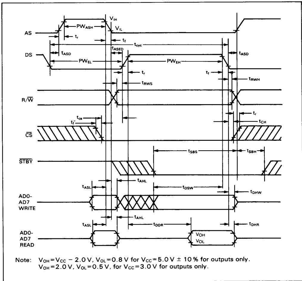
Figure 19. Bus Read, Write Timing (6801 Family)
