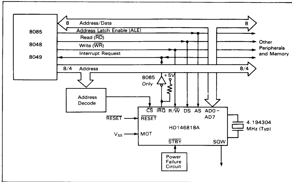
Figure 17. HD146818A Interface with 8085 Family Microprocessors
