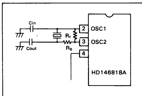
Figure 13. Note for Board Design of the Oscillation Circuit (1)
