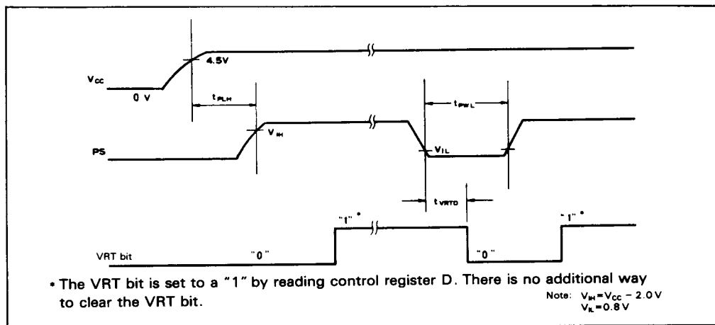
Figure 24. VRT Bit Clear Timing
