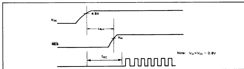
Figure 25. Power Up Timing
