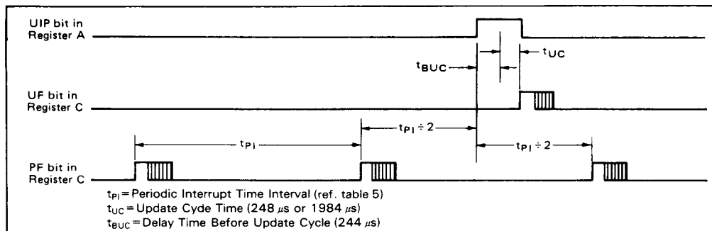
Figure 11. Update-Ended and Periodic Interrupt Relationship
