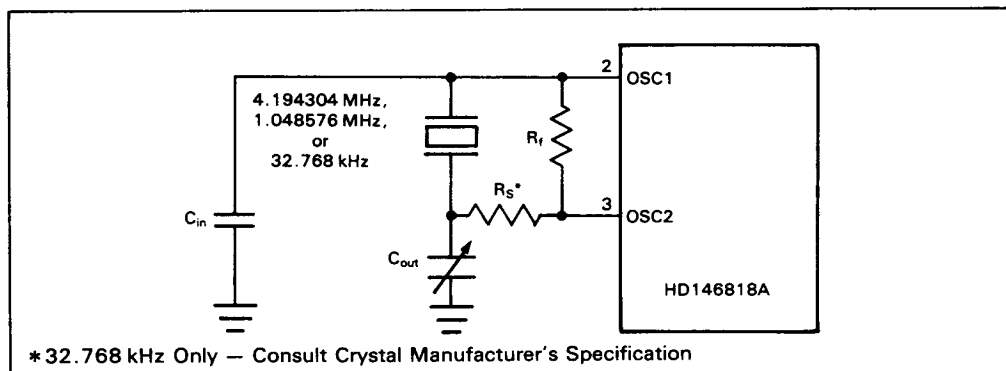
Figure 12. Crystal Oscillator Connection
