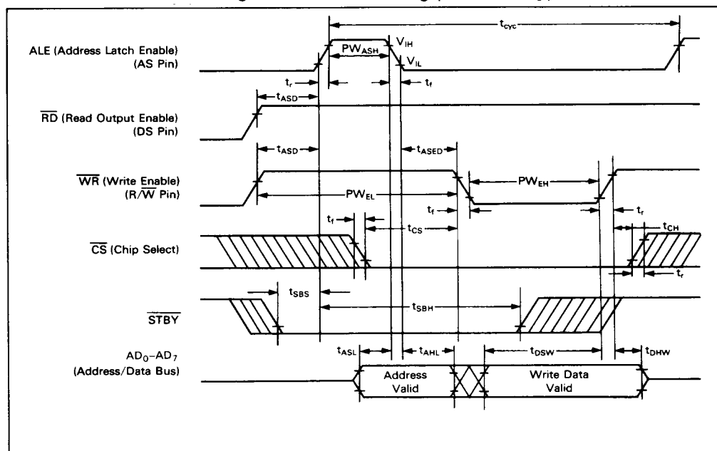
Figure 21. Write Timing (8085 Family)
