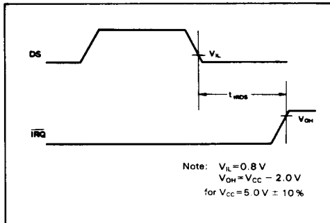
Figure 22. \overline{\text{IRQ}} Release Delay (from DS)
