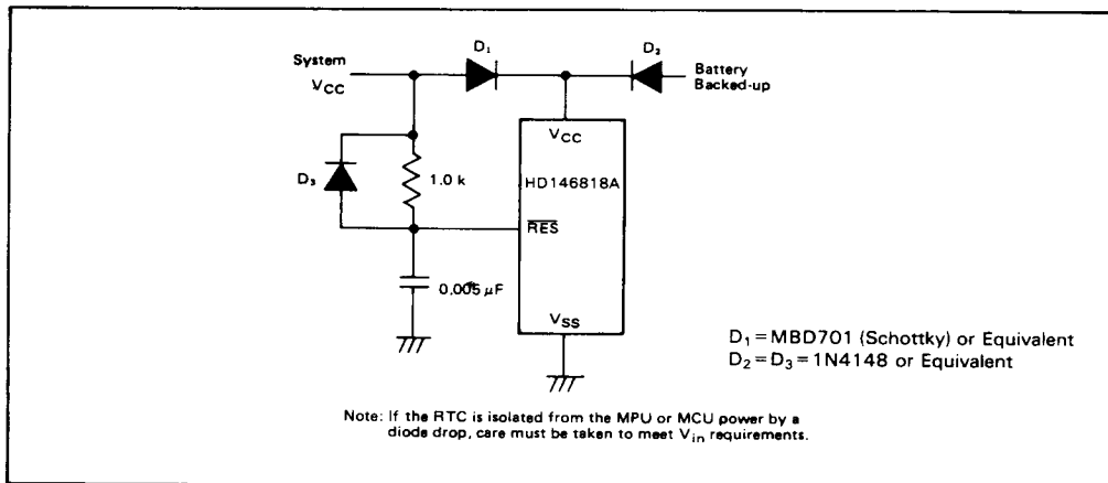
Figure 2. Typical Powerup Delay Circuit for RES
