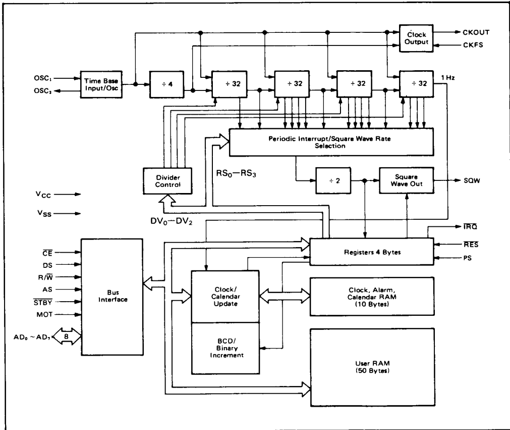
Figure 4. Block Diagram
