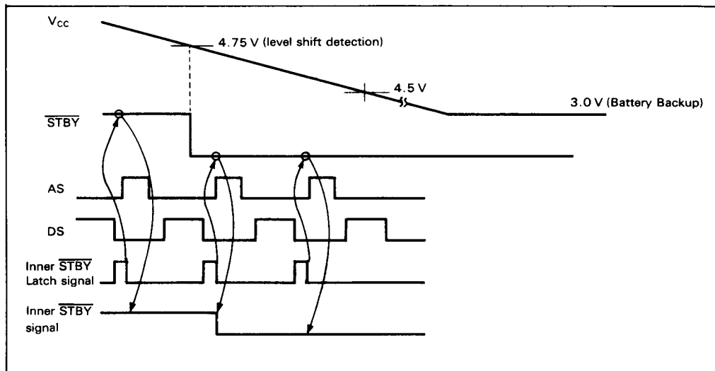
Figure 15. Battery Backup Timing example
