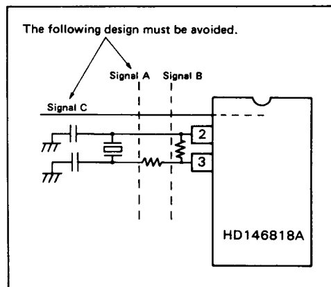
Figure 14. Note for Board Design of the Oscillation Circuit (2)
