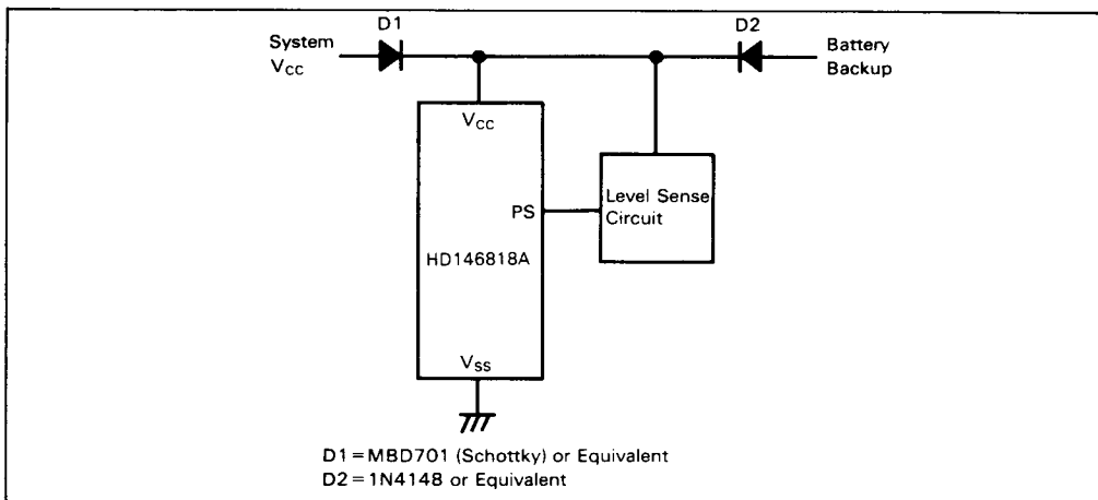
Figure 3. Typical Powerup Delay Circuit for Power Sense
