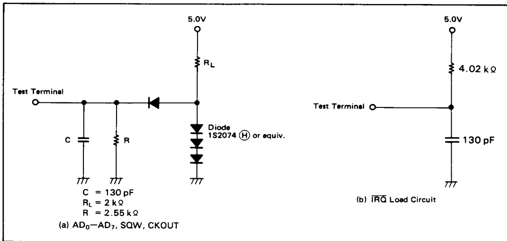
Figure 26. Test Load
