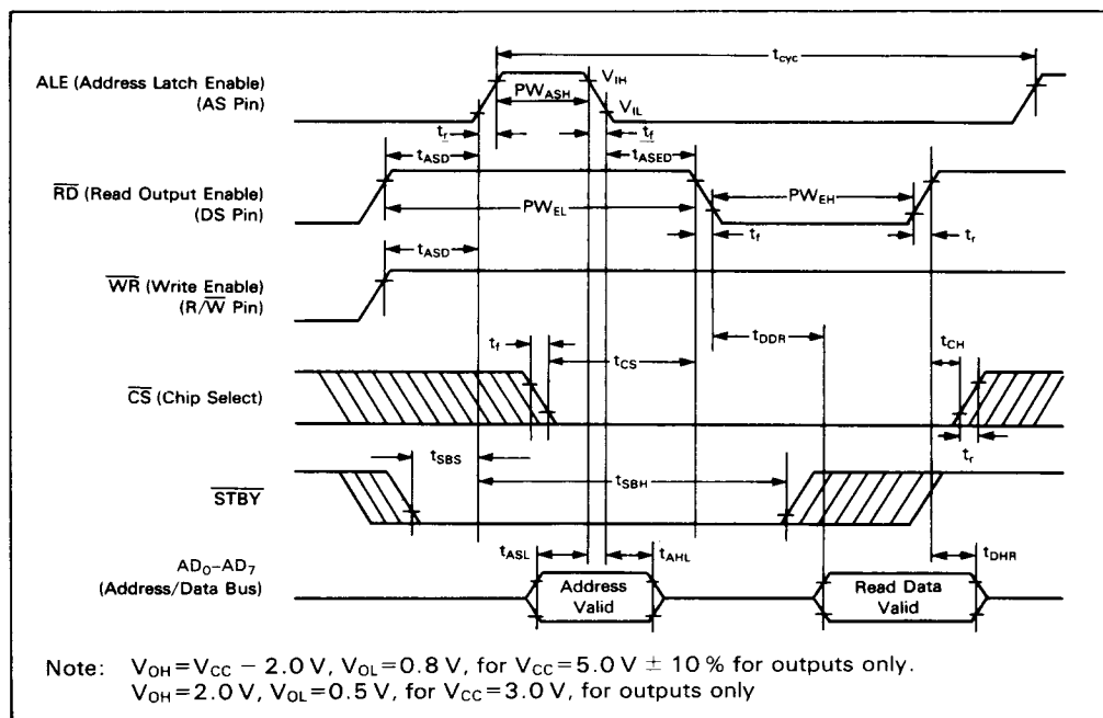
Figure 20. Read Timing (8085 Family)
