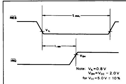
Figure 23. \overline{\text{IRQ}} Release Delay (from RES)
