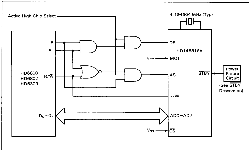
Figure 18. HD146818A Interface with 6800 Family Microprocessors
