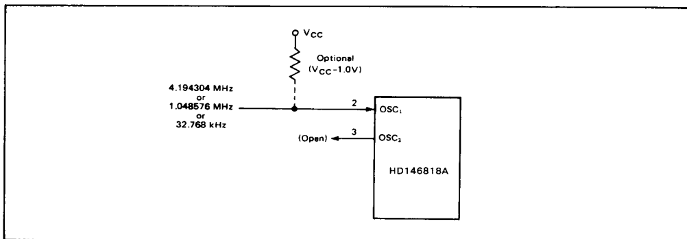
Figure 1. External Time-Base Connection
