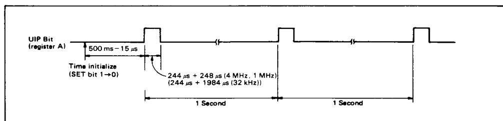
Figure 10. Time Initialization and the First Update
