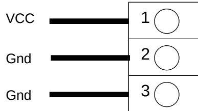
FIGURE 2-3 P6: +5V Power Connector
