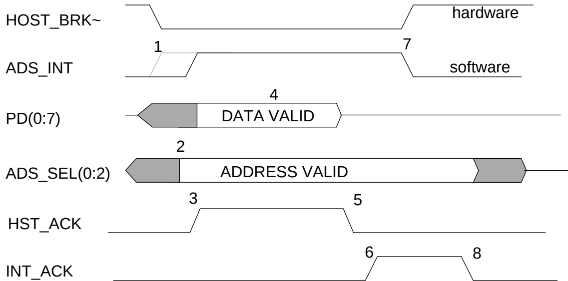
FIGURE B-4 M68360QUADS-040 Interrupt to Host
