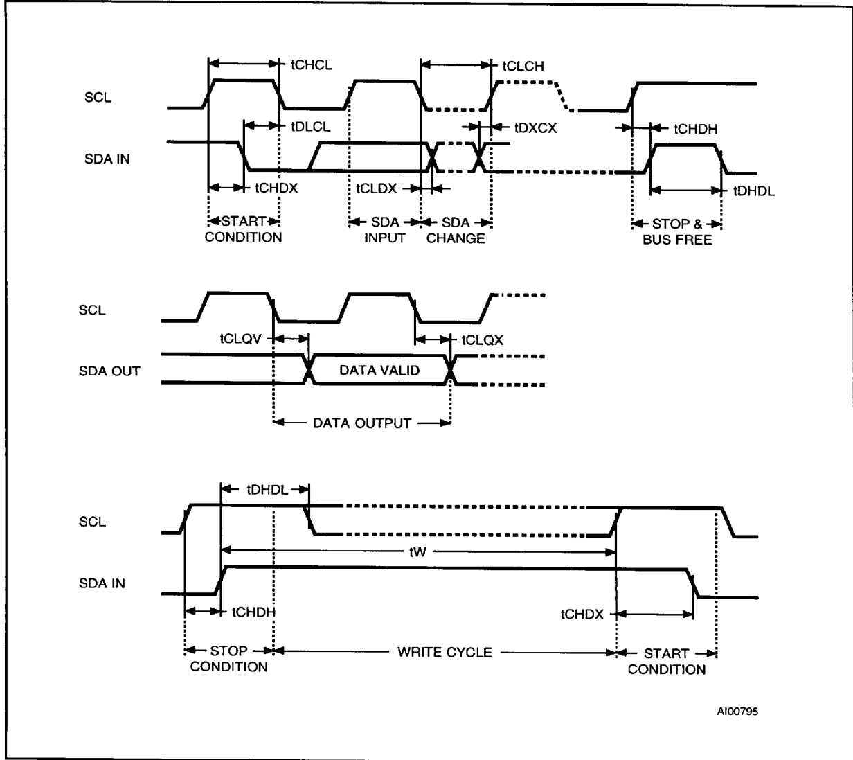
Figure 5. AC Waveforms
