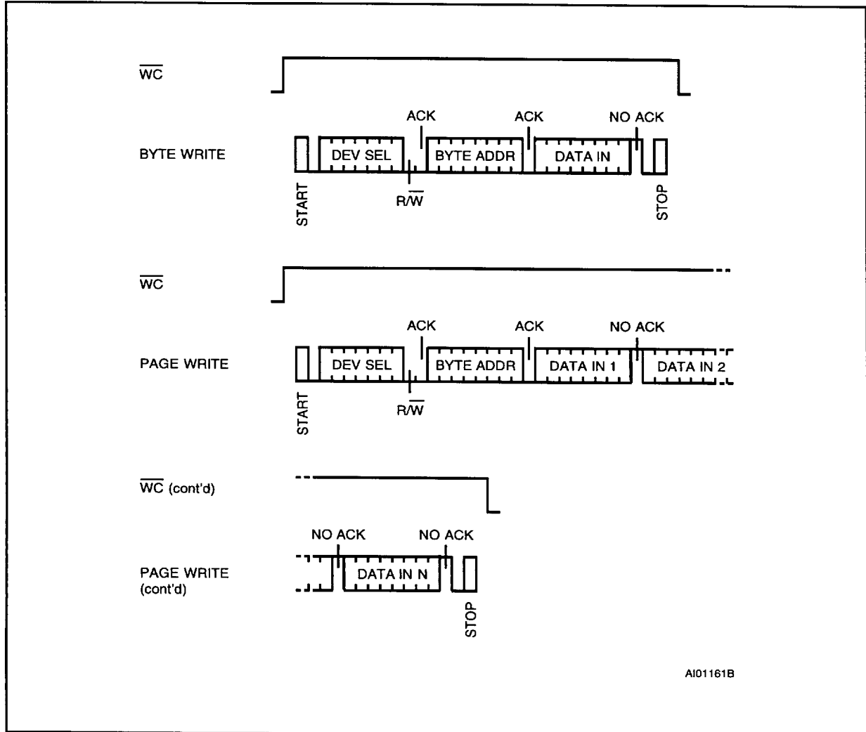
Figure 10. Write Modes Sequence with Write Control = 1 (ST24/25W08)
