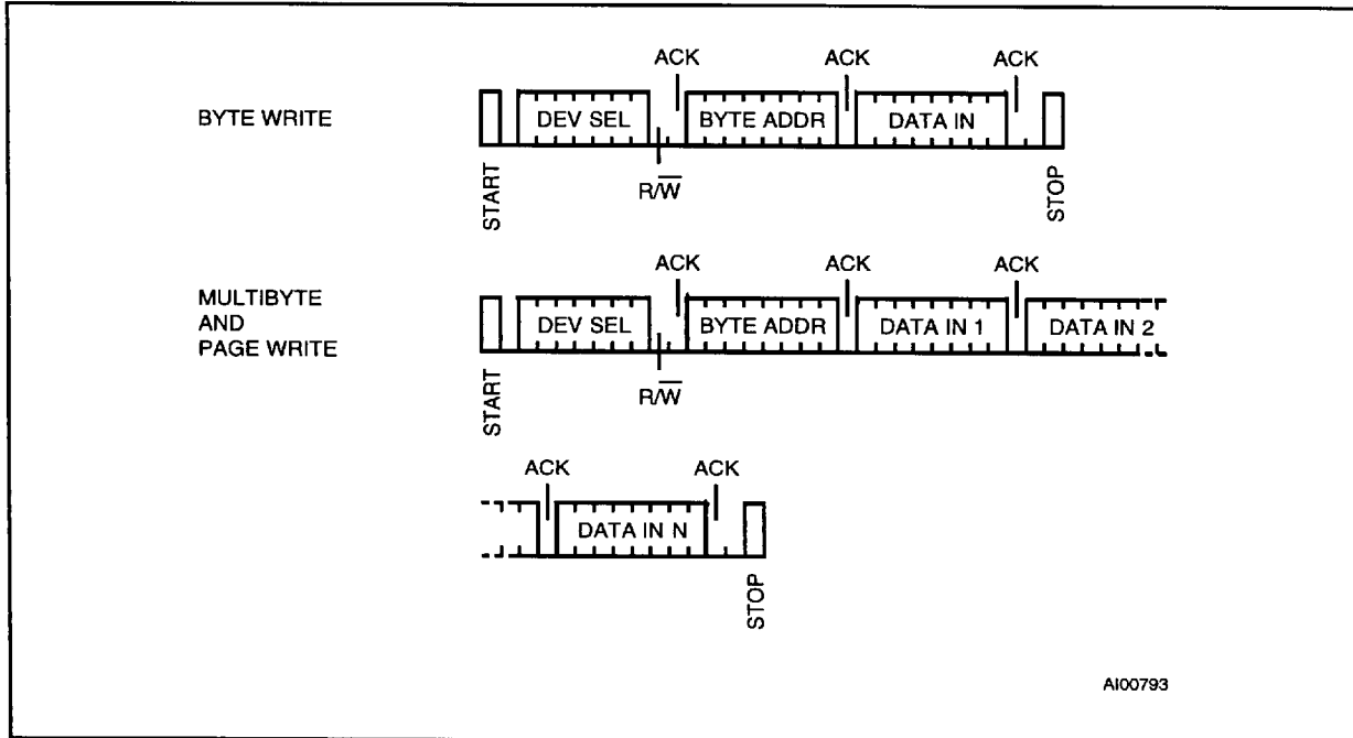
Figure 9. Write Modes Sequence (ST24/25C08 and ST24C08R)
