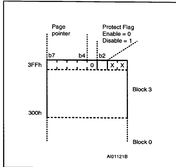
Figure 7. Memory Protection
