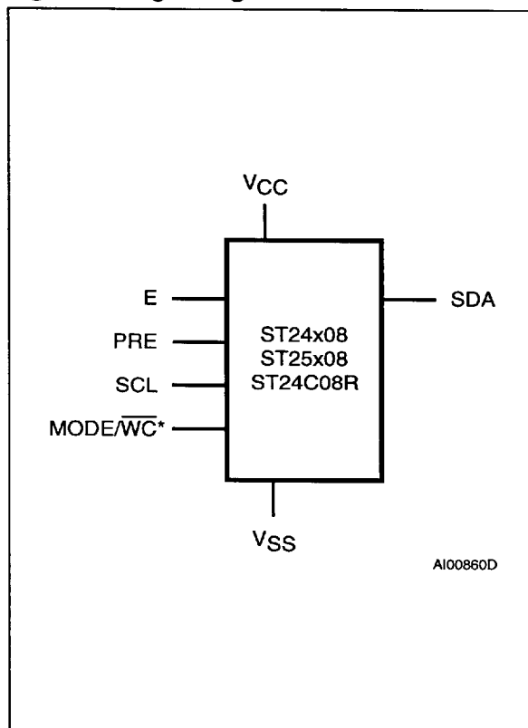
Figure 1. Logic Diagram
