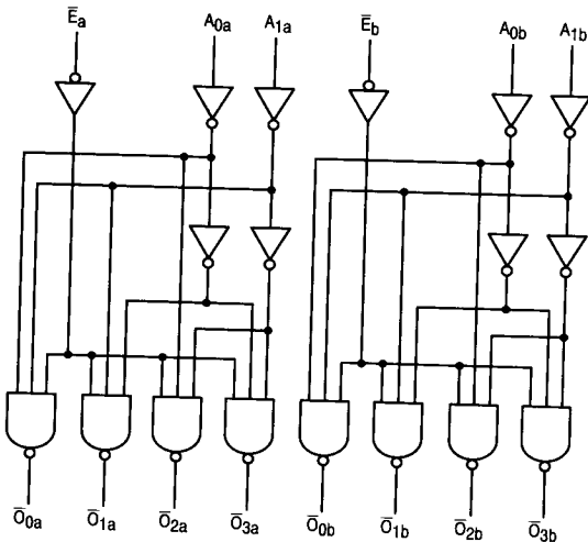
LOGIC DIAGRAM
