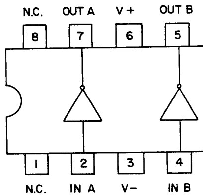
FIGURE 1. Terminal connections and logic diagrams.
