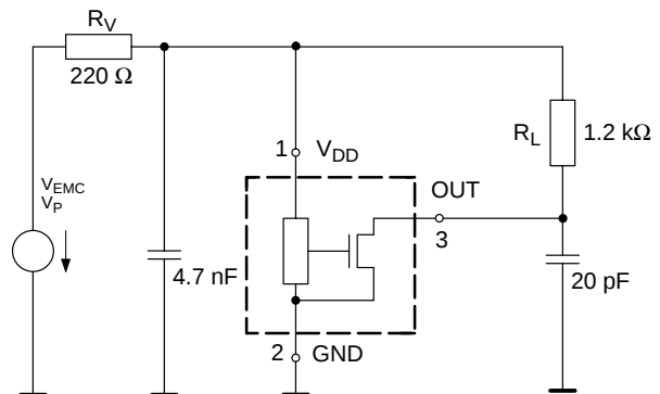
Fig. 5–2: Test circuit 2
