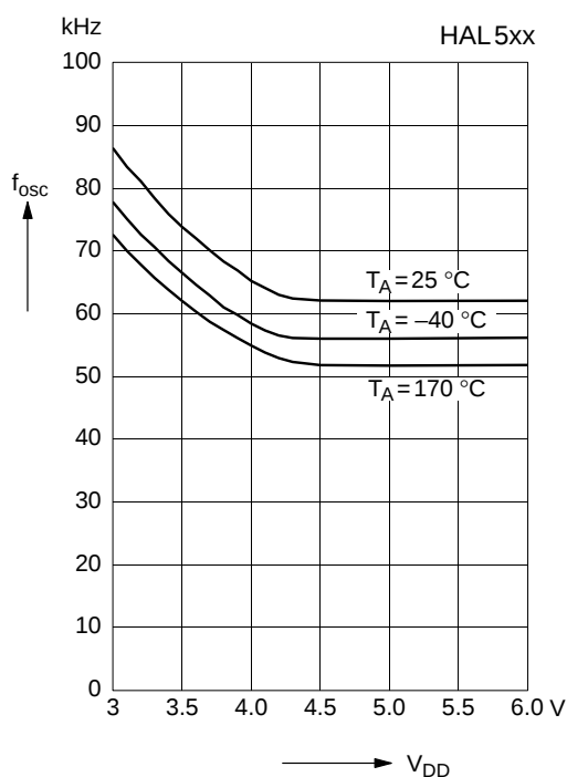
Fig. 3-10: Typ. internal chopper frequency versus supply voltage
