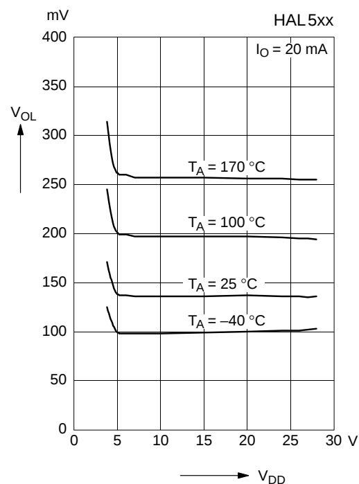
Fig. 3-11: Typical output low voltage versus supply voltage
