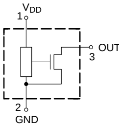
Fig. 1–1: Pin configuration
