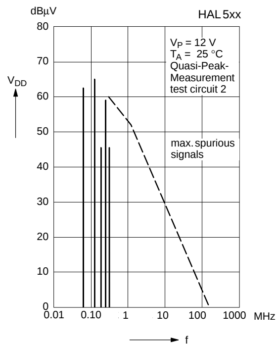
Fig. 3-17: Typ. spectrum at supply voltage
