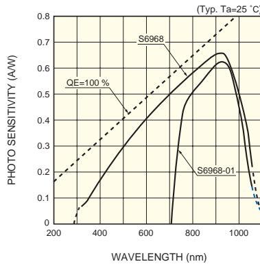
S6968 series
