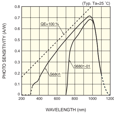
S6801 series
