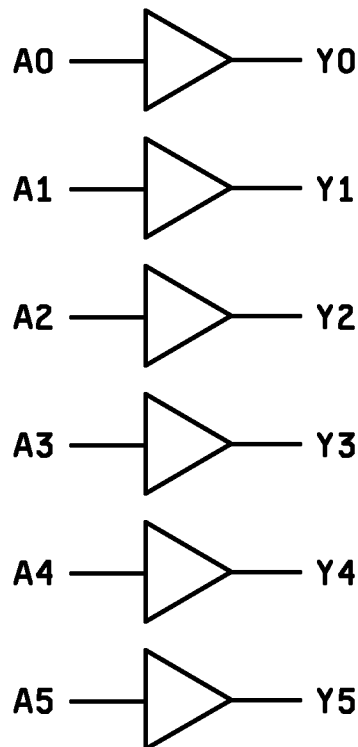
FIGURE 3. Logic diagram.
