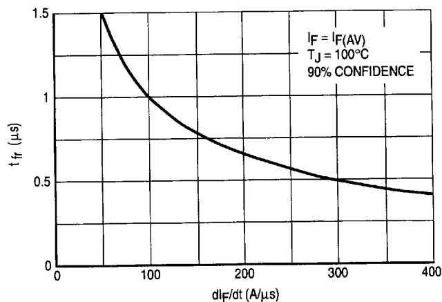
Figure 7. Recovery Time versus di_F/dt
