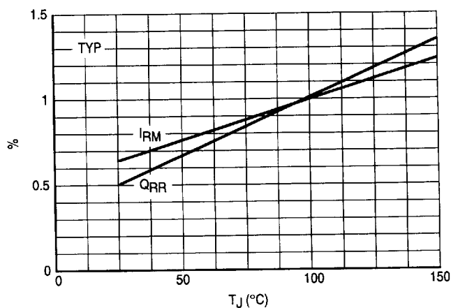
Figure 10. Dynamic Parameters versus Junction Temperature
