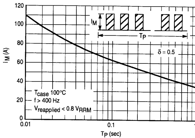
Figure 3. Non-Repetitive Peak Surge Current versus Overload Duration
