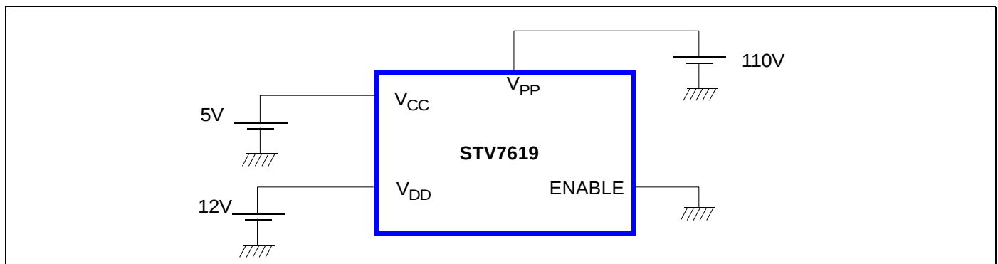
Figure 4: External Power Supply (Large-size PDP)
