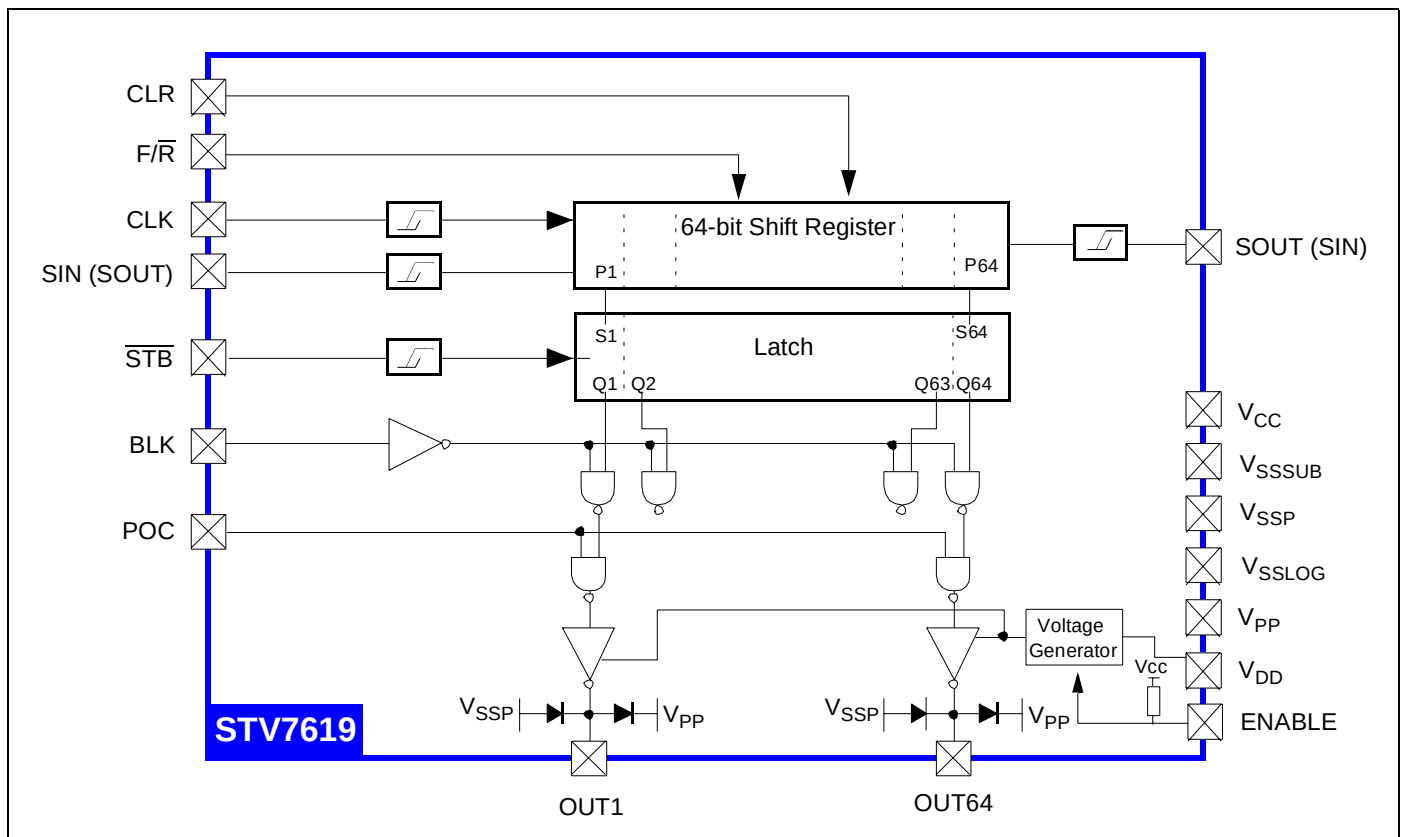
Figure 2: Block Diagram
