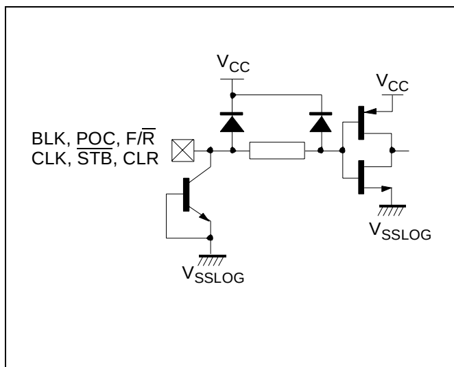
Figure 10: F/R, CLR, CLK, STB, BLK and POC Inputs
