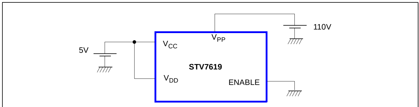
Figure 3: External Power Supply (Small-size PDP)
