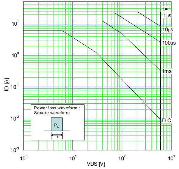
Safe Operating Area I_D = f(V_{DS}) : Duty=0 (Single pulse), T_c = 25\text{ }^\circ\text{C}
