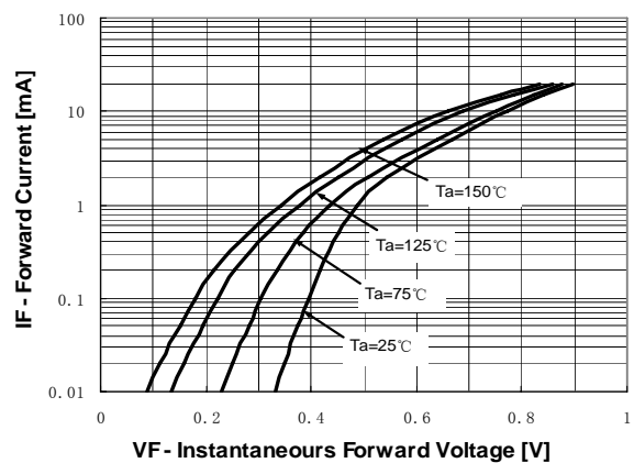
Figure 6. MBRF20100CT Typical Forward Voltage (Per Diode)
