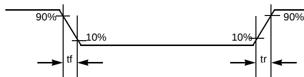
Figure 1. Switching Characteristics
