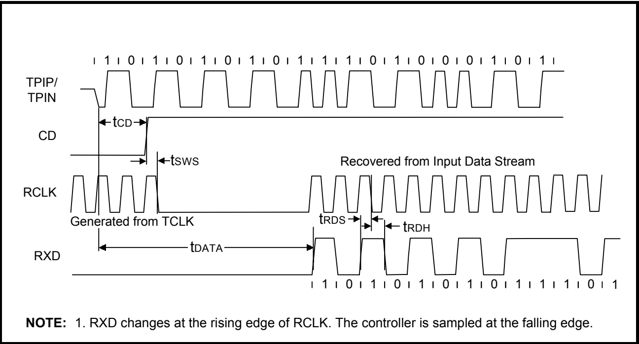
Figure 27: Mode 3 RCLK/Start-of-Frame Timing
