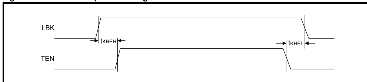
Figure 20: Mode 1 Loopback Timing
