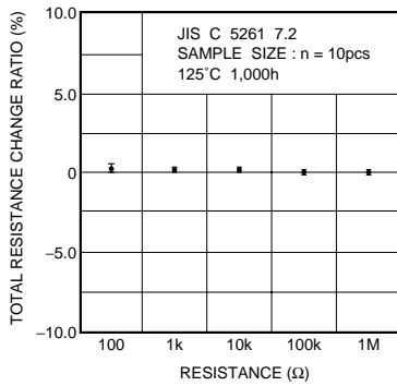
Fig.9 Resisance to dry heat
