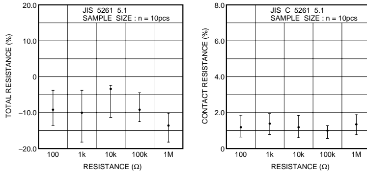
Fig.3 DC resistance : Total and contact
