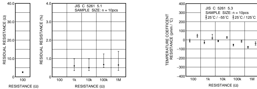
Fig.4 Residual resistance
