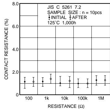
Fig.9 Resisance to dry heat
