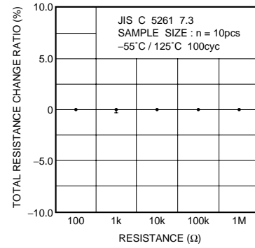
Fig.10-1 Temperature cycling
