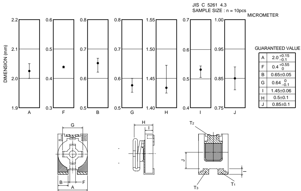
Fig.2 Dimensions
