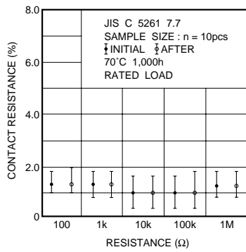
Fig.13-2 Endurance (rated load)
