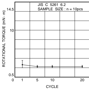
Fig.7 Rotational torque
