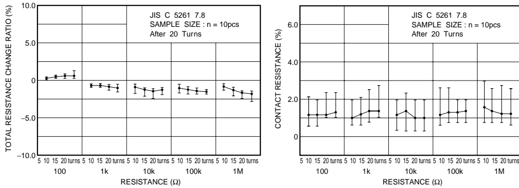
Fig.6-1 Endurance (wiper)
