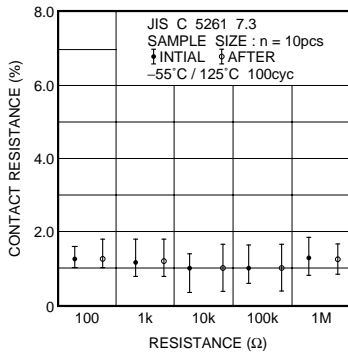
Fig.10-2 Temperature cycling
