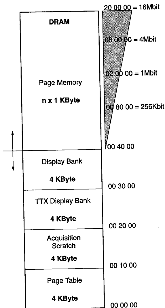
Fig. 4-8: Memory Organization
