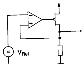
Fig. 3-5: Supply Pin 1
