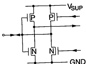
Fig. 3-7: Input/Output Pins 3 to 14, 18, 25, 26
