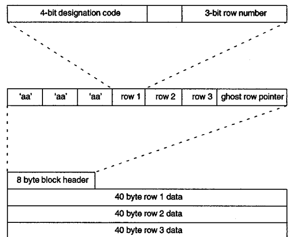
Fig. 4-11: Ghost Block Structure
