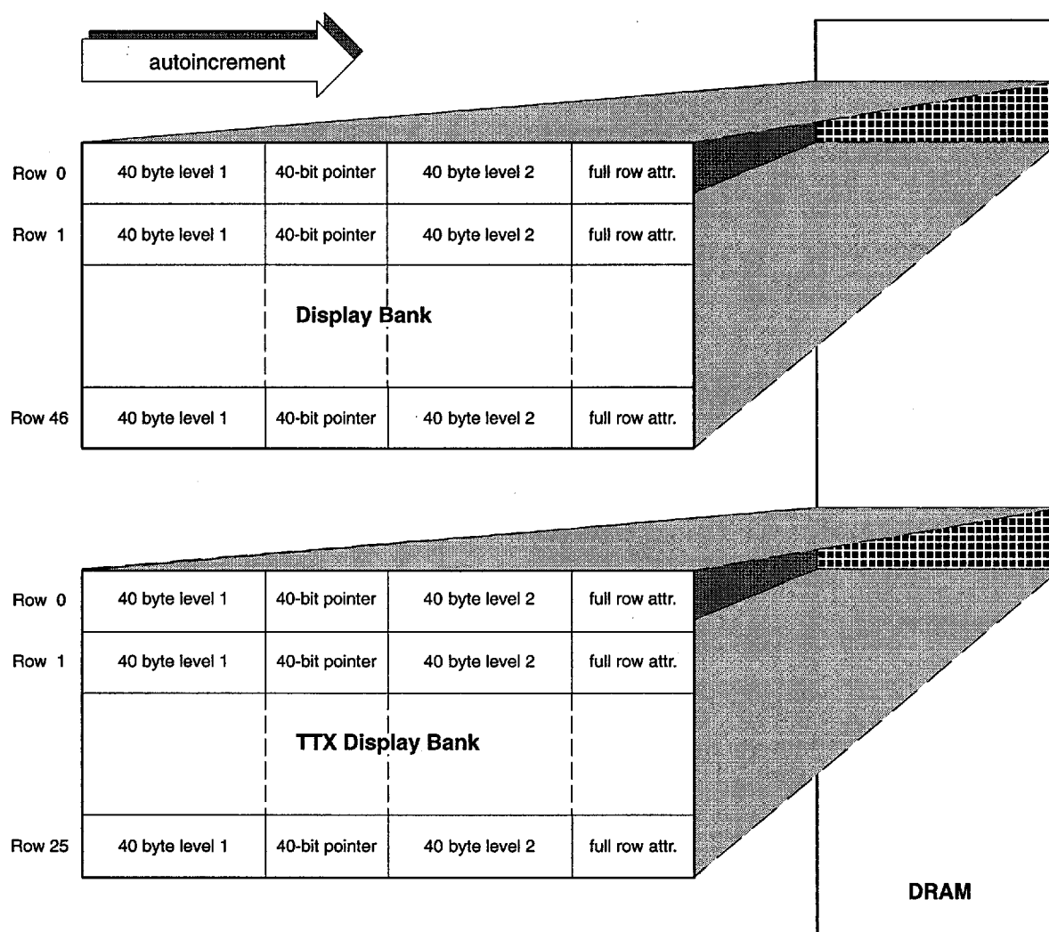
Fig. 4-4: Display Memory Organization
