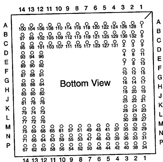
Fig. 6-1: EMU 3040 in 132-pin PGA package
