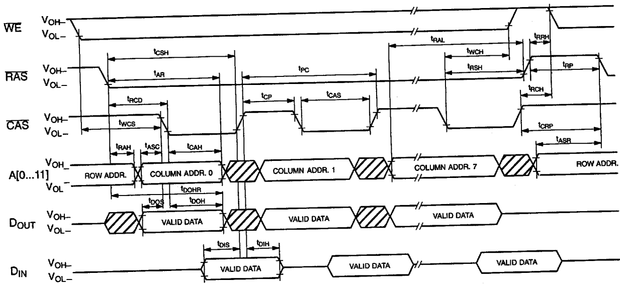
Fig. 3-15: DRAM page mode waveforms
