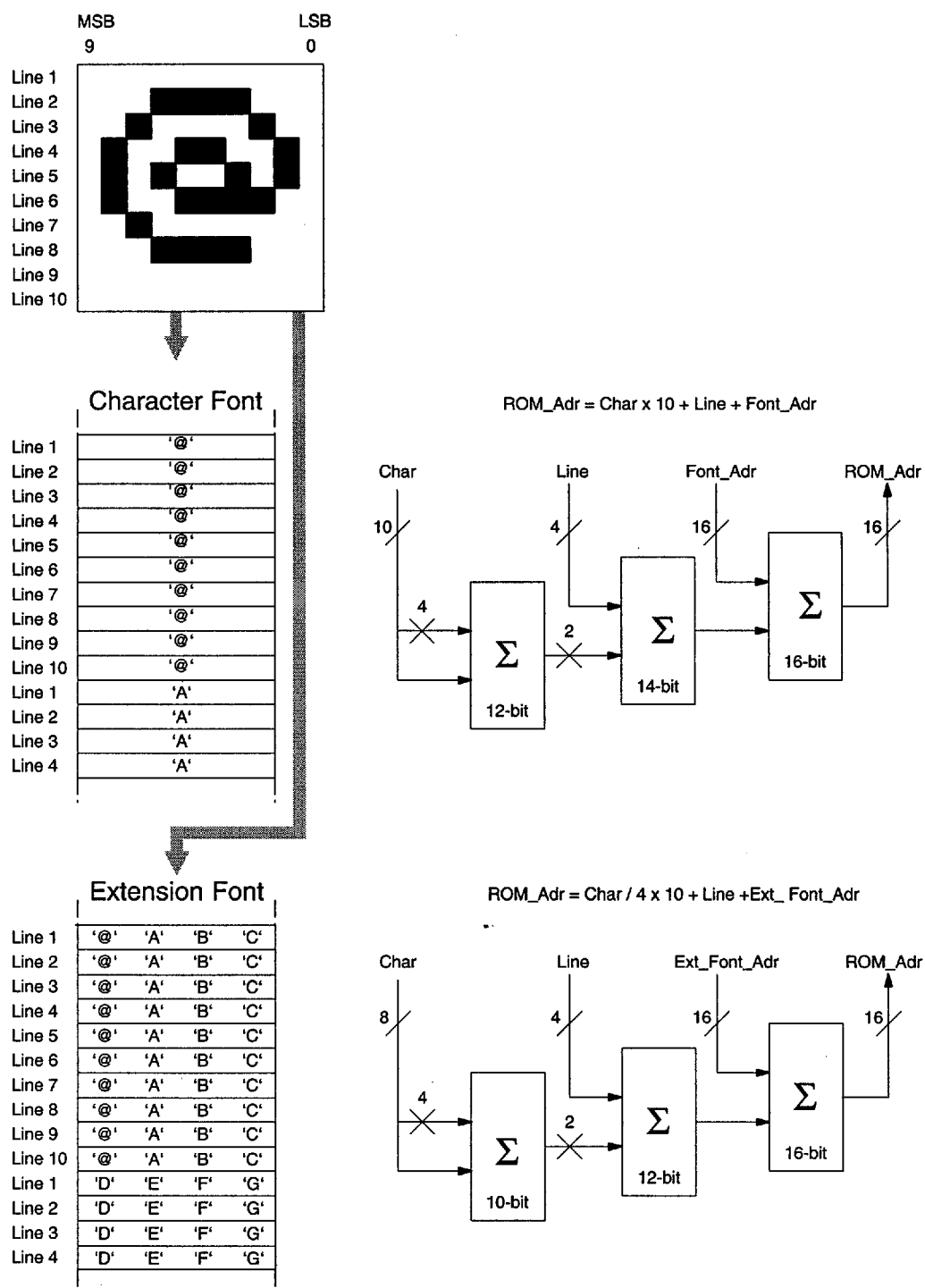
Fig. 4-6: Character Font Structure
