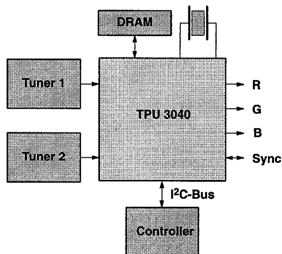
Fig. 2-4: Stand-Alone Application
