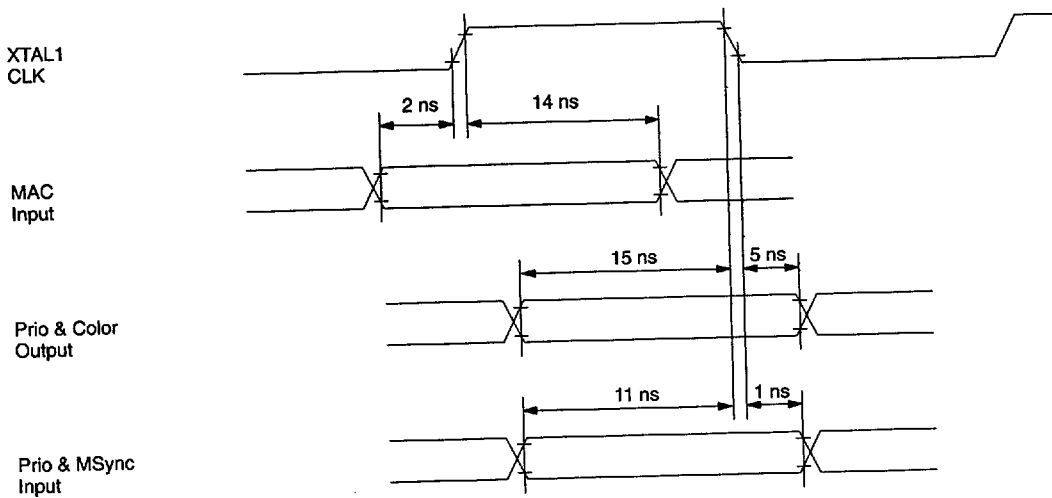
Fig. 3-16: TPU 3040 Timing
