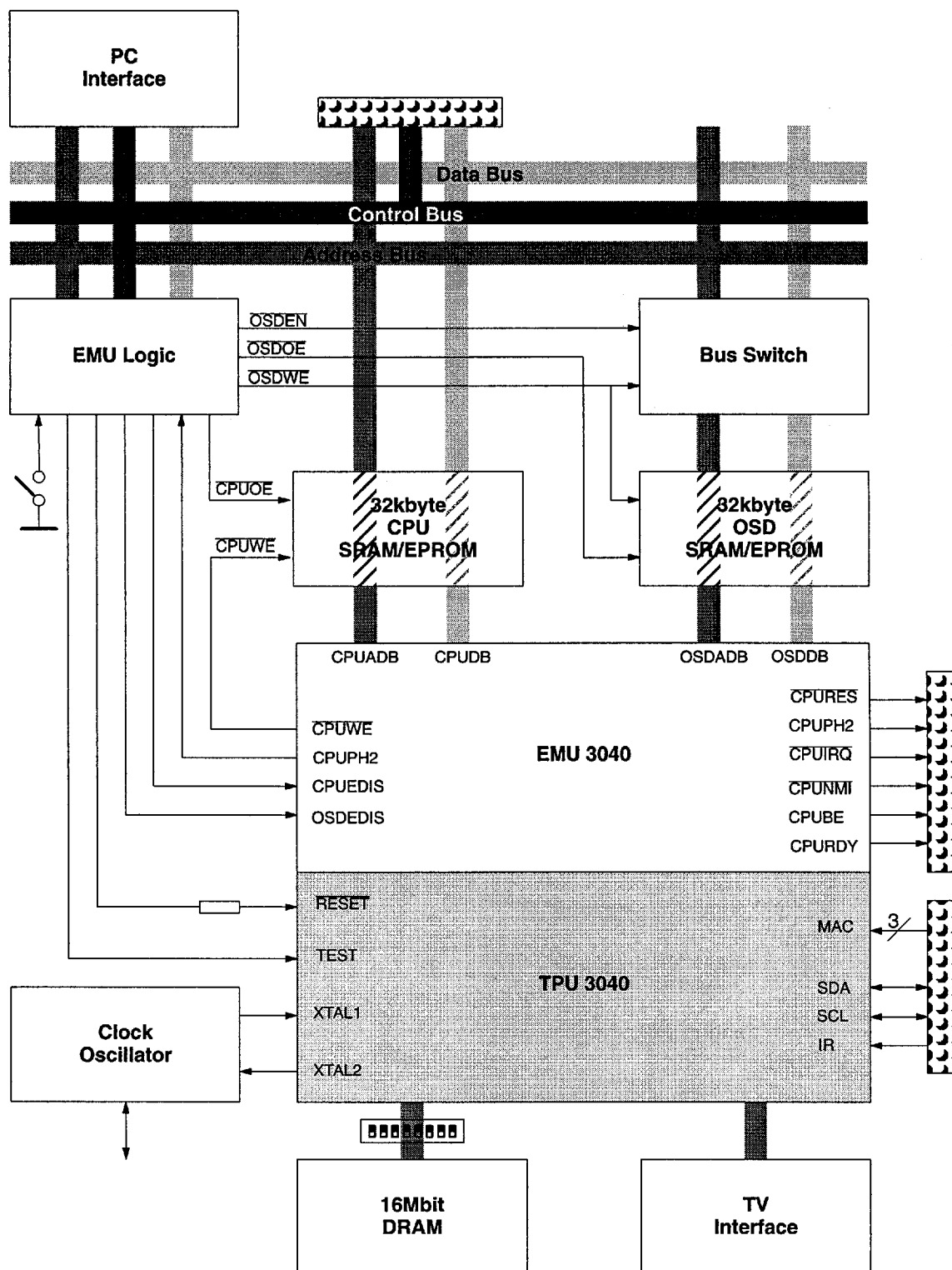
Fig. 6-2: EMU 3040 Board
