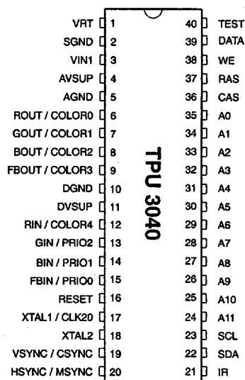
Fig. 3–3: TPU 3040 in 40-pin PDIP package
