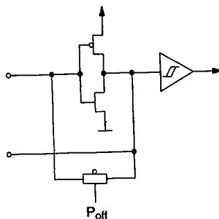
Fig. 3-11: Output/Input Pins 27, 28
