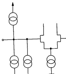
Fig. 3-14: Input Pins 42 and 44
