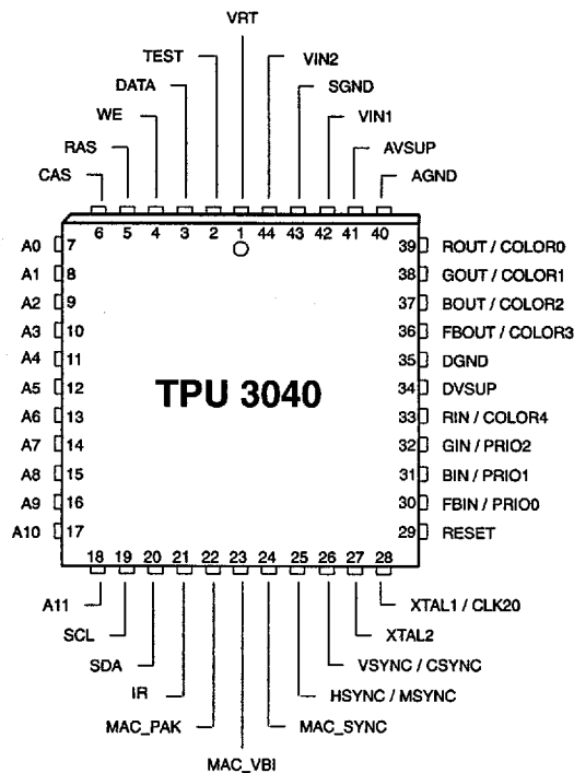
Fig. 3–4: TPU 3040 in 44-pin PLCC package
