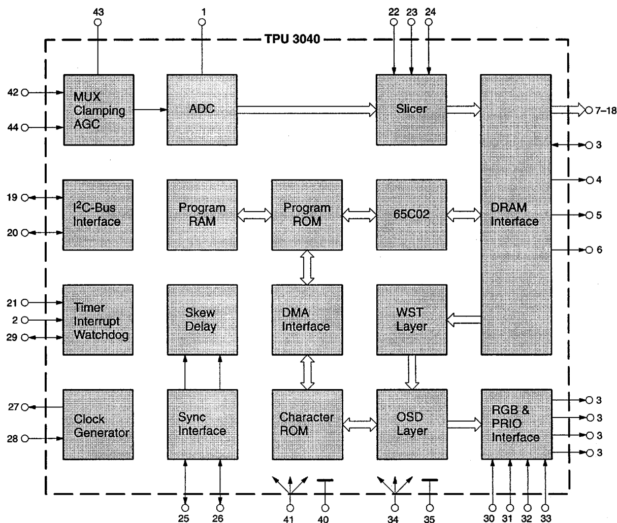
Fig. 2-1: Functional block diagram of TPU 3040
