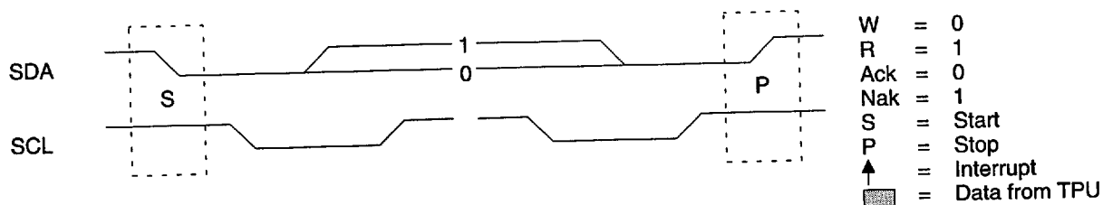
Fig. 4-3: I 2 C-bus Protocol
