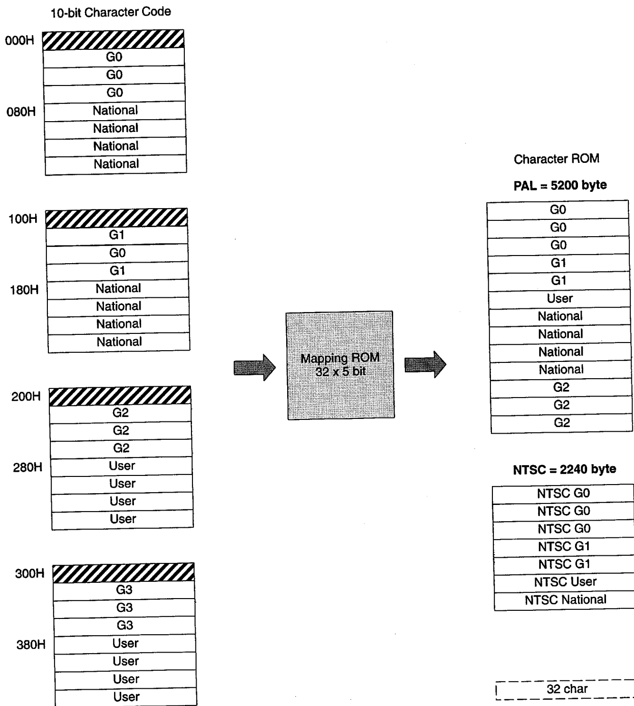
Fig. 4-5: Character Set Organisation
