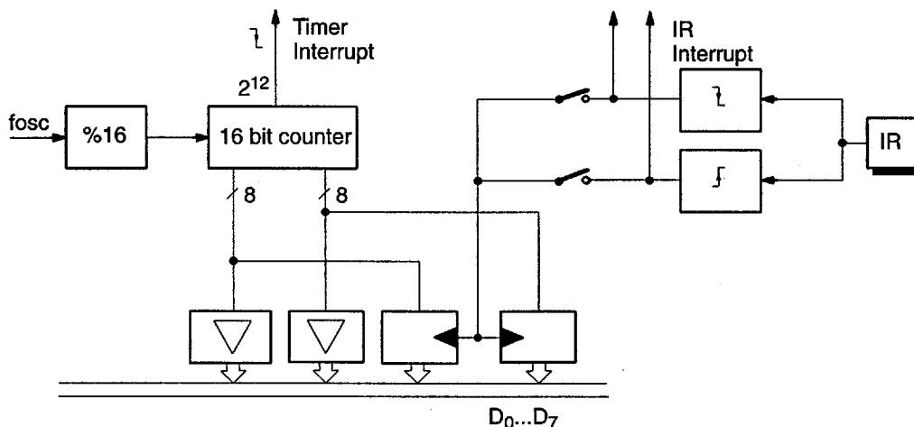
Fig. 2-5: Timer Structure
