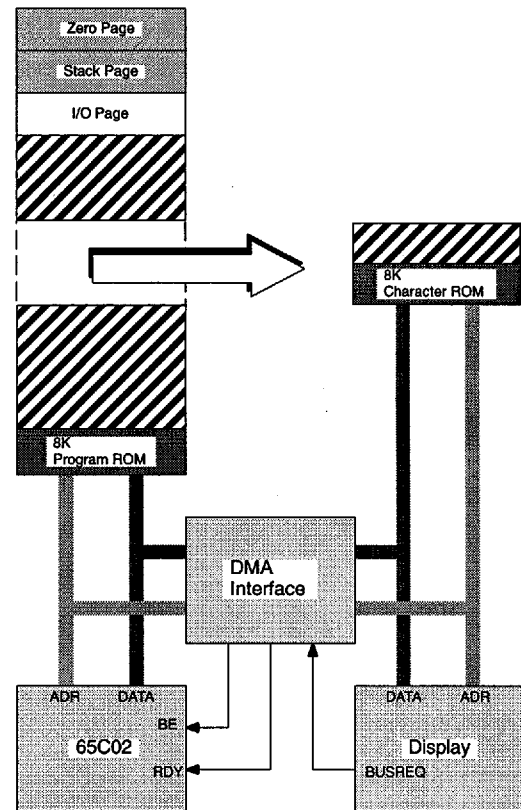
Fig. 4-1: 65C02 memory environment
