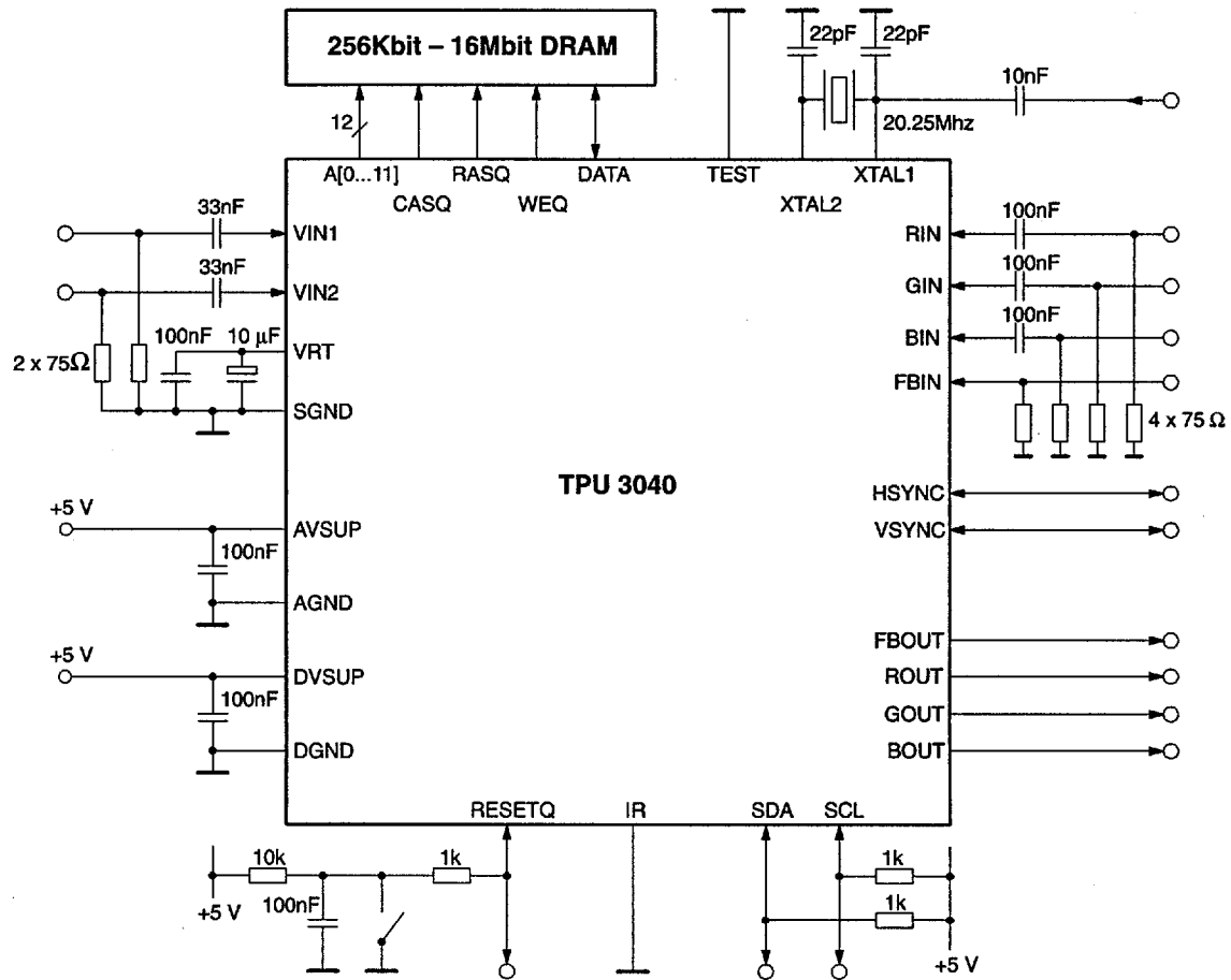
Fig. 5-1: TPU 3040 Application
