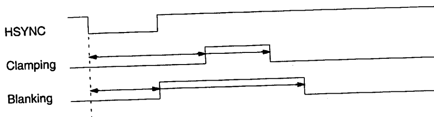
Fig. 2-6: Internal Timing
