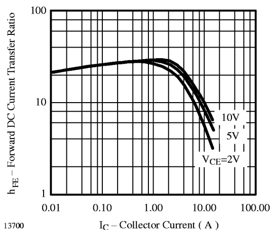
Figure 6. h_{\text{FE}} vs. I_C
