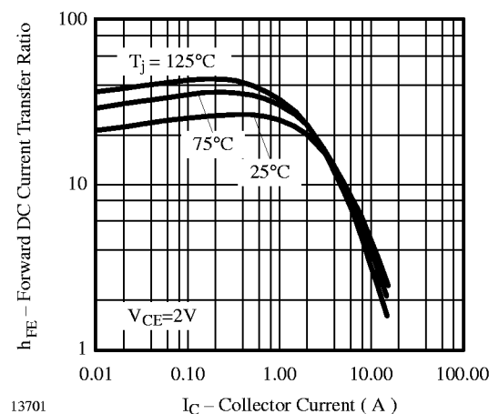
Figure 9. h_{\text{FE}} vs. I_C
