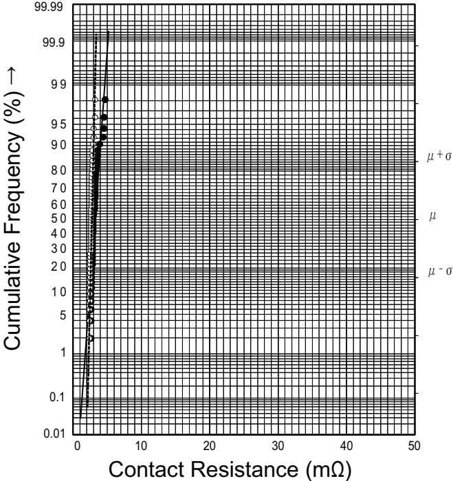
2. Contact Resistance Distribution
