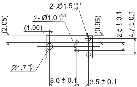
Mounting hole layout (bottom view)
