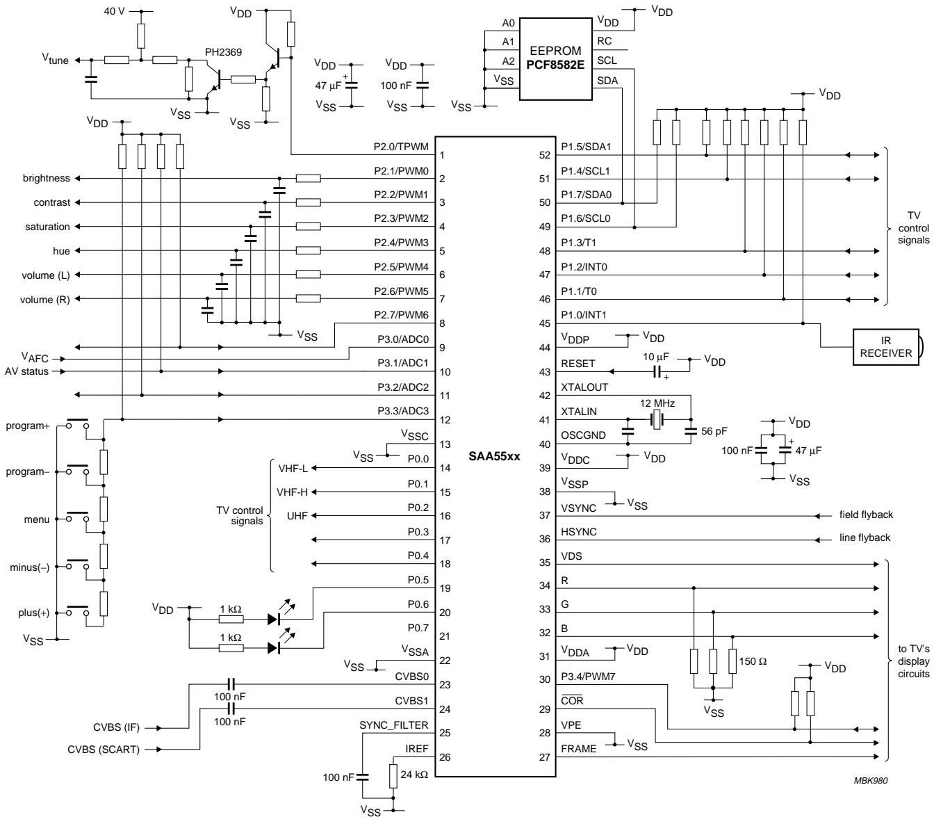
Fig.40 Application diagram.
