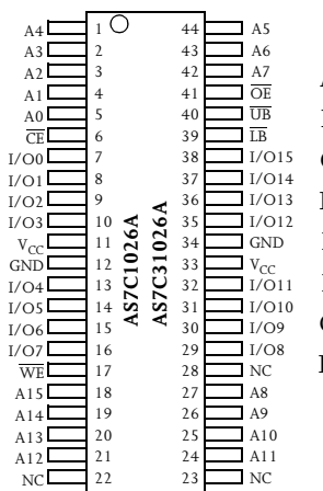
44-Pin SOJ (400 mil), TSOP 2
