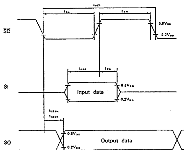
Fig. 4 Serial transfer timing
