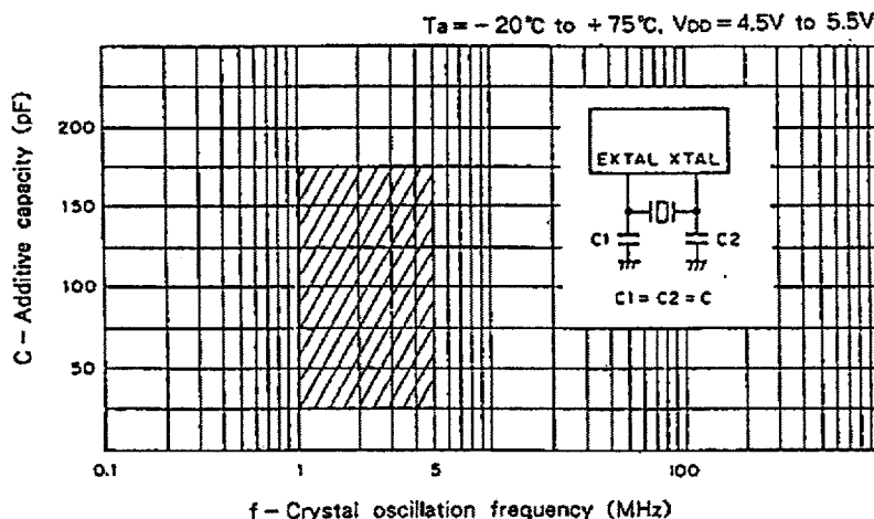
Fig. 11 Crystal oscillation circuit additive capacity calculation chart
