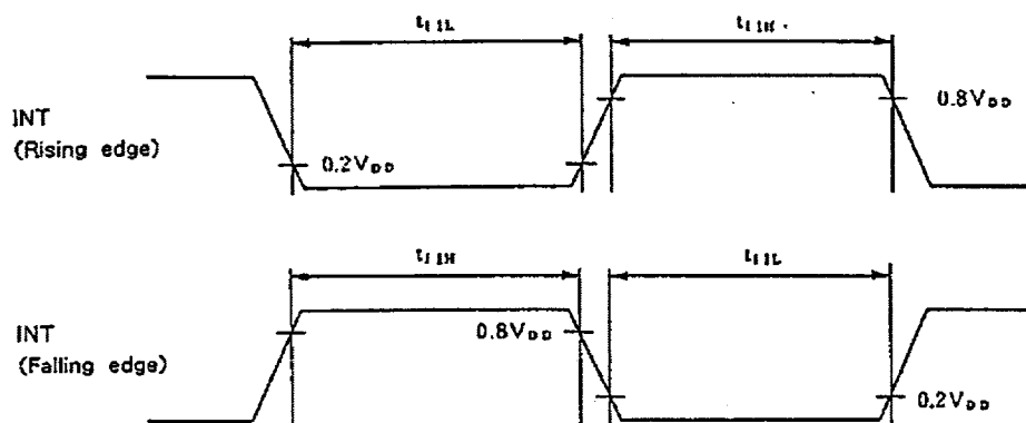
Fig. 6 Interruption input timing
