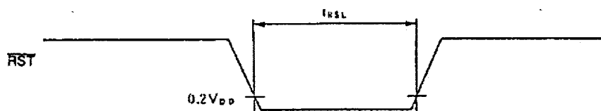
Fig. 7 Reset input timing
