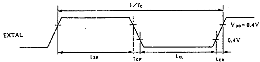
Fig. 1 Clock timing
