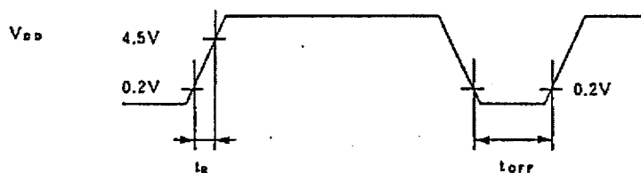
Fig. 10 Power on reset
