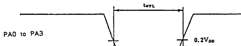
Fig. 9 Wake-up input timing
