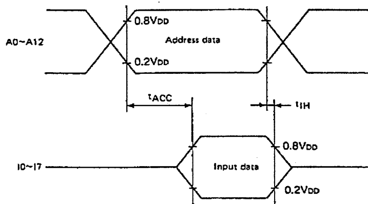
Fig. 14 EPROM timing
