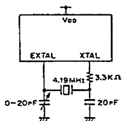
Fig. 12 Frequency adjustment circuit
