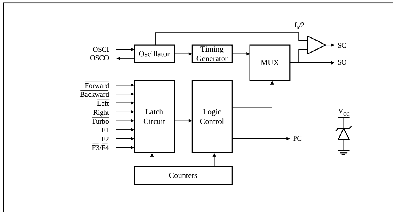
Figure 1. Block Diagram of PT8A9701P
