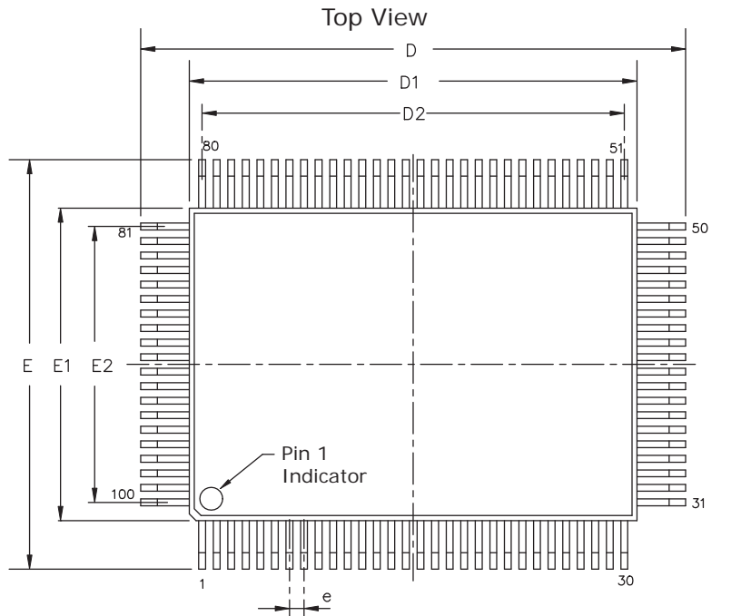
Figure 12. Package Drawing
