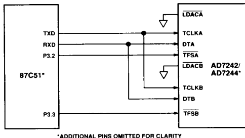
Figure 10. AD7242/AD7244 to 87C51 Interface
