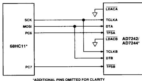
Figure 11. AD7242/AD7244 to 68HC11 Interface
