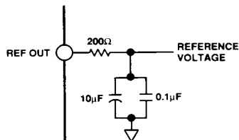
Figure 2. Circuit Connection for REF OUT with an External Capacitive Load of Greater Than 50\text{ pF}
