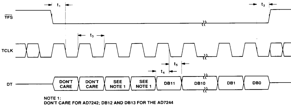
Figure 6. AD7242/AD7244 Timing Diagram
