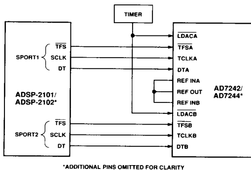
Figure 7. AD7242/AD7244 to ADSP-2101/ADSP-2102 Interface
