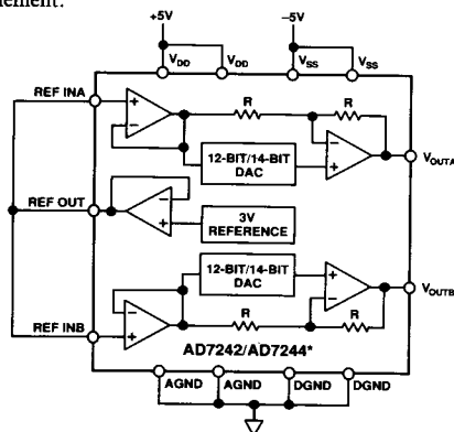
Figure 5. Basic Connection Diagram
