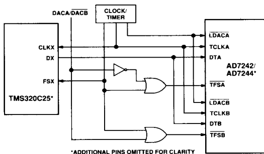
Figure 9. AD7242/AD7244 to TMS320C25 Interface
