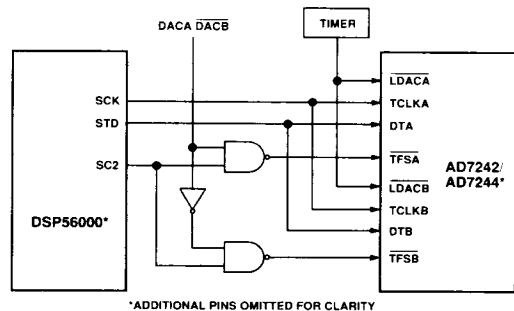
Figure 8. AD7242/AD7244 to DSP56000 Interface
