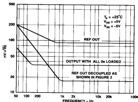
Figure 4. Noise Spectral Density vs. Frequency
