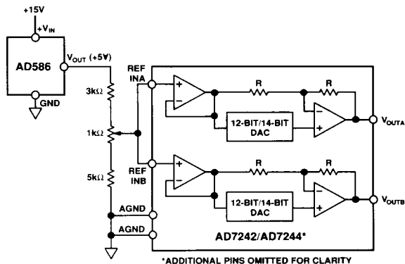
Figure 3. AD586 Driving AD7242/AD7244 Reference Inputs
