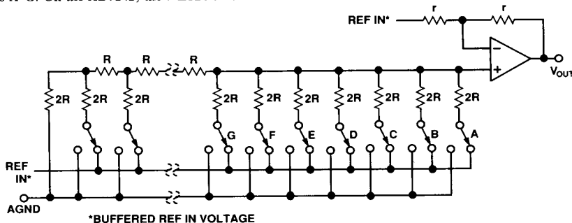
Figure 1. DAC Ladder Structure
