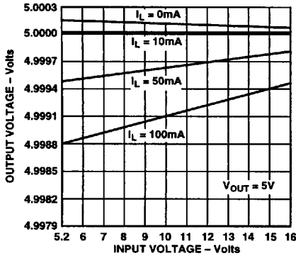
Figure 2. Line Regulation: Output Voltage vs. Input Voltage
