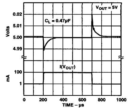
Figure 13. Load Transient for 1 mA to 100 mA Pulse
