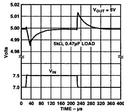
Figure 12. Line Transient Response
