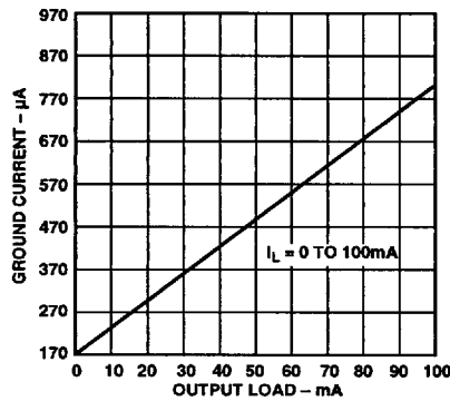
Figure 5. Quiescent Current vs. Load Current
