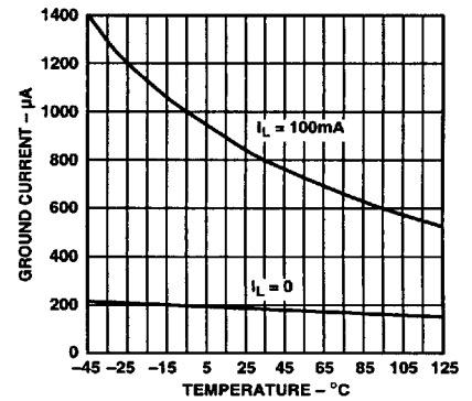
Figure 7. Quiescent Current vs. Temperature
