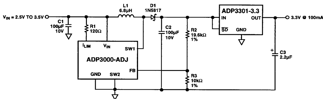
Figure 23. Step-Up/Step-Down Post Regulator
