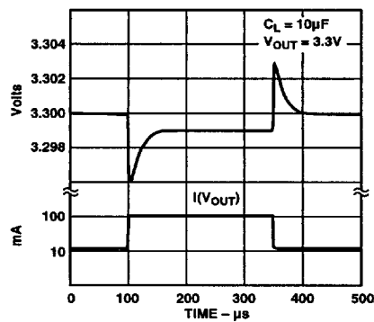
Figure 14. Load Transient for 10 mA to 100 mA Pulse
