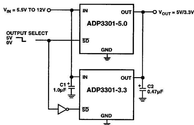
Figure 21. Crossover Switch
