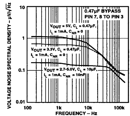
Figure 19. Output Noise Density
