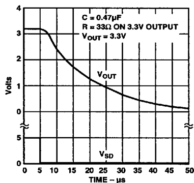
Figure 17. Turn-Off
