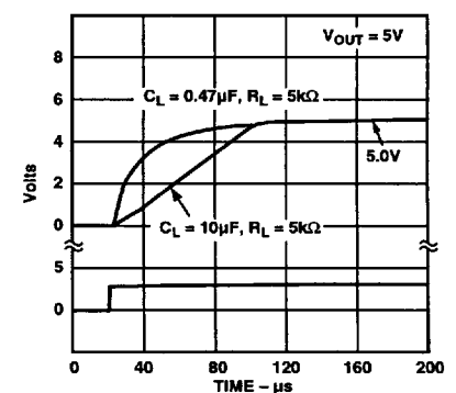
Figure 16. Turn-On
