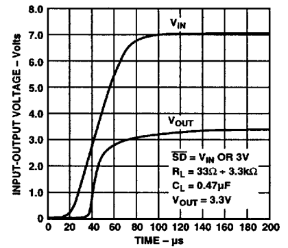
Figure 10. Power-Up Overshoot
