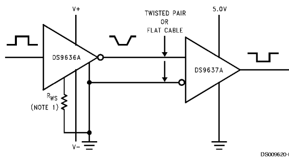
FIGURE 2. RS-423 System Application
