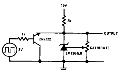
5.0V Square Wave Calibrator
