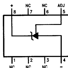
SO Package
