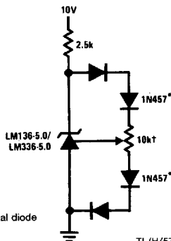
5.0V Reference with Minimum Temperature Coefficient
