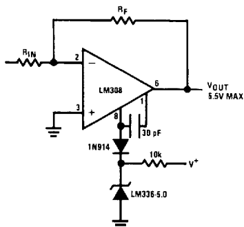
Op Amp with Output Clamped
