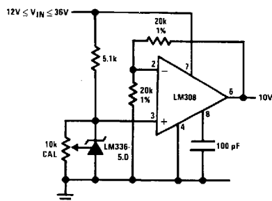
Wide Input Range Reference
