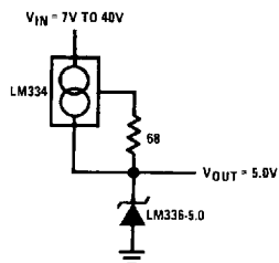
Wide Input Range Reference
