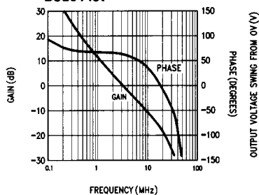
Bode Plot
