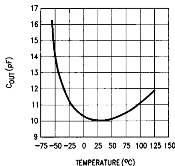
FIGURE 7. I_{OL} and C_{OUT} vs Temperature
