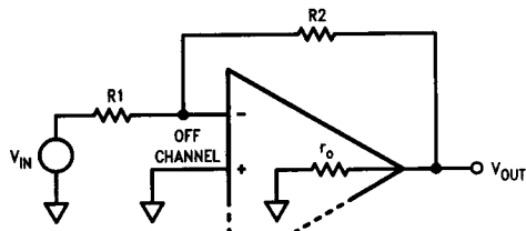
FIGURE 11. Inverting Gain Channel Feedthrough
