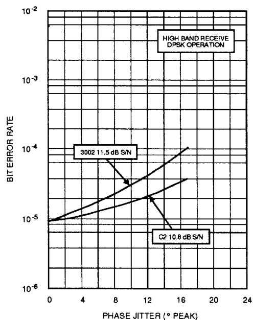
*SSI 73K222AL BER vs PHASE JITTER
