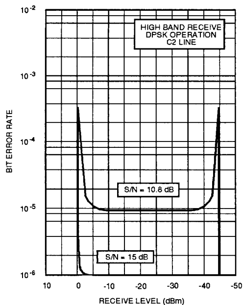
*SSI 73K222AL BER vs RECEIVE LEVEL
