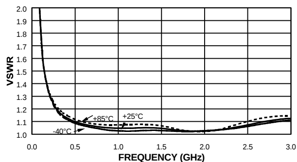
VSWR Over Temperature
