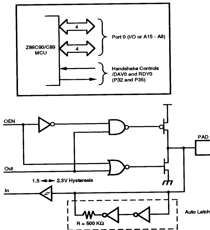
Figure 5. Port 0 Configuration
