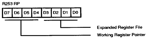
Figure 42. Register Pointer (FD H :Read/Write)
