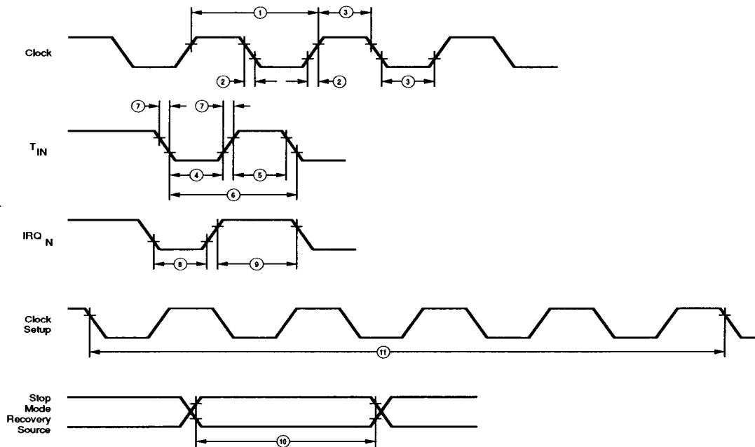
Figure 24. Additional Timing
