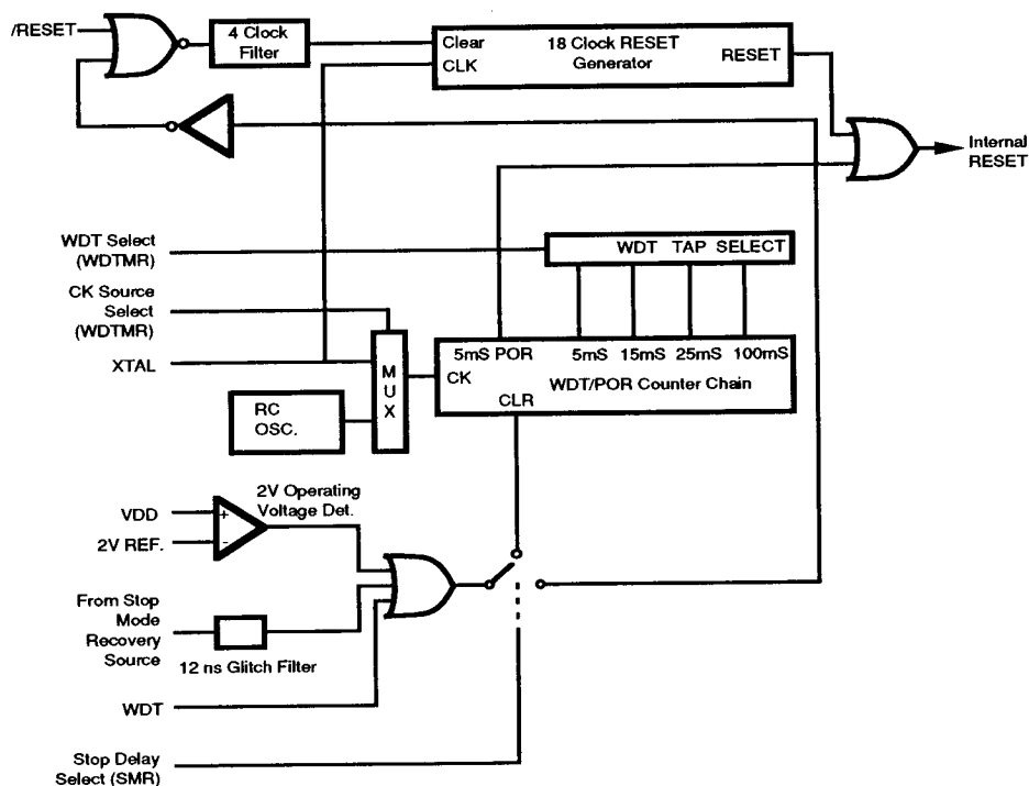
Figure 20. Resets and WDT
