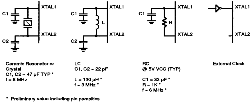
Figure 16. Oscillator Configuration
