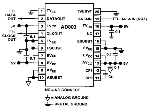
Application/Test Circuit
