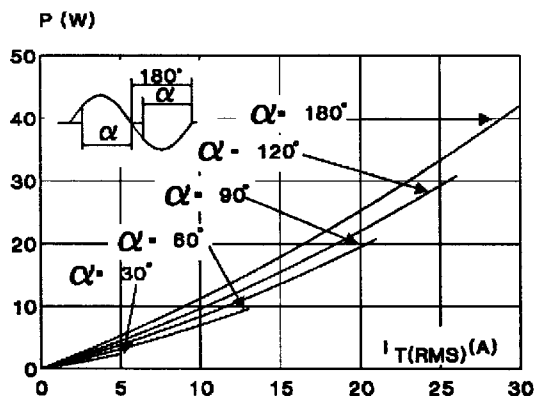
Fig.3 : Maximum RMS power dissipation versus RMS on-state current ( F=50\text{Hz} ). (Curves are cut off by (di/dt)_c limitation) (BTB)
