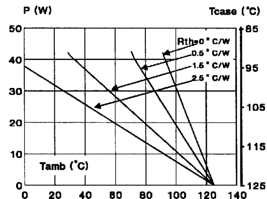
Fig.4 : Correlation between maximum RMS power dissipation and maximum allowable temperatures ( T_{\text{amb}} and T_{\text{case}} ) for different thermal resistances heatsink + contact (BTB).
