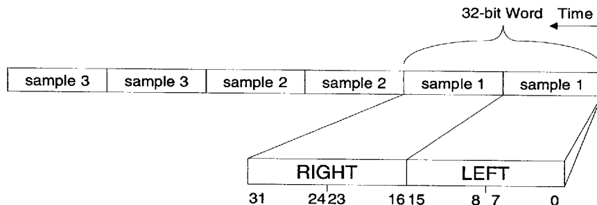
Figure 17. 16-bit Stereo, Signed Little Endian Audio Data
