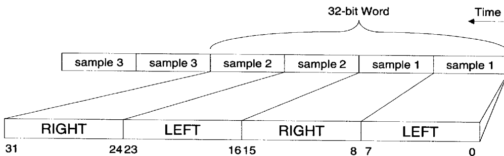
Figure 15. 8-bit Stereo, Unsigned Audio Data
