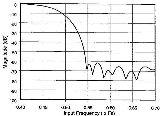
Figure 39. DAC Transition Band
