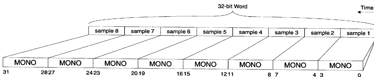
Figure 18. 4-bit Mono, ADPCM Audio Data
