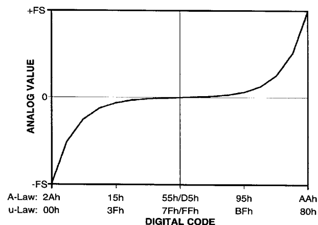
Figure 23. Companded Transfer Functions
