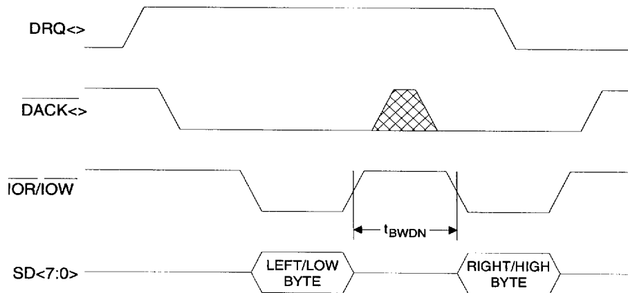
8-Bit Stereo or 16-Bit Mono DMA Cycle
