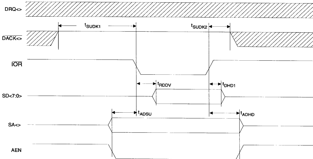
I/O Read Cycle
