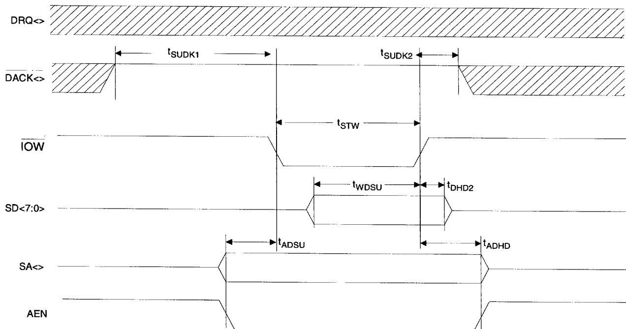
I/O Write Cycle
