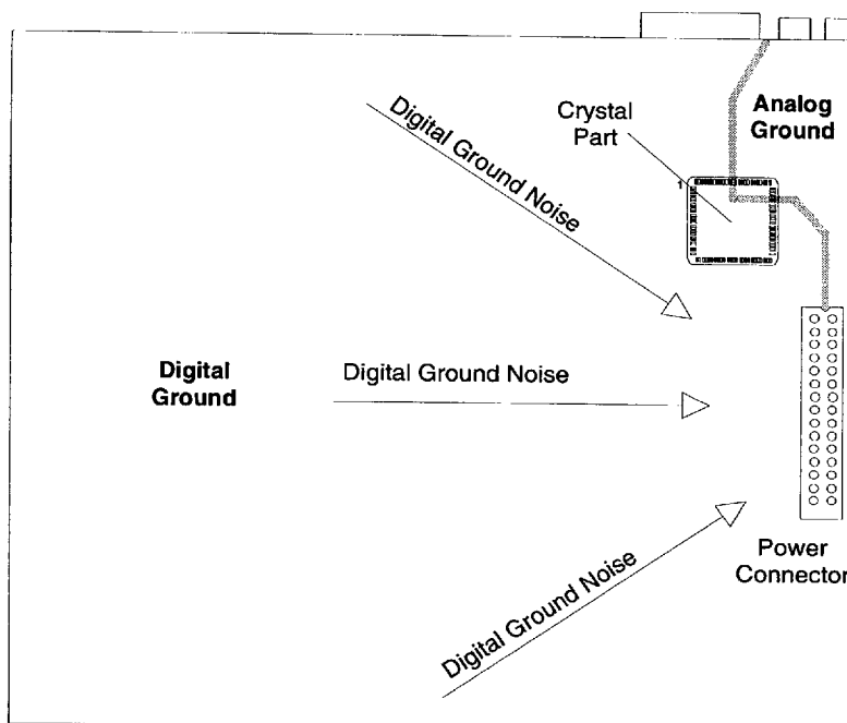
Figure 31. Suggested Motherboard Layout
