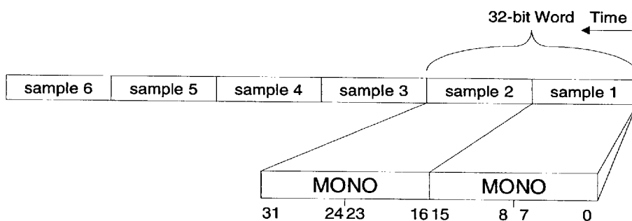
Figure 16. 16-bit Mono, Signed Little Endian Audio Data
