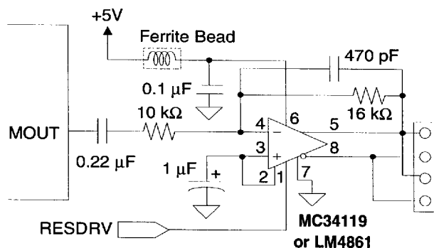
Figure 30. Mono Output
