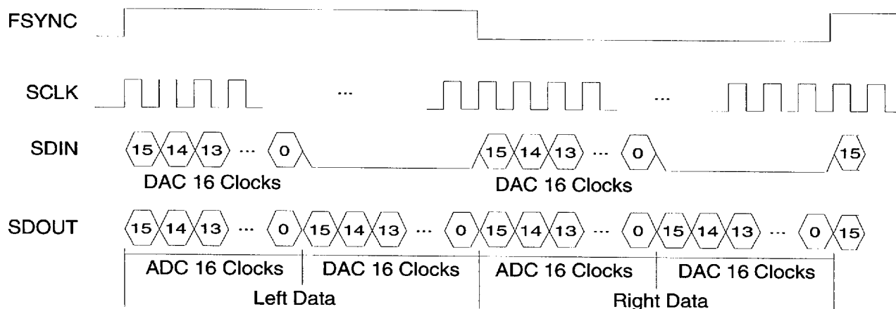
Figure 12. ADC/DAC Mode (SF1,0 = 11)
