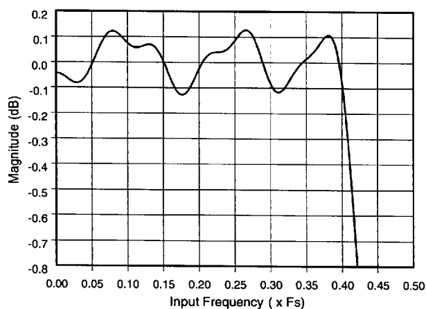
Figure 38. DAC Passband Ripple
