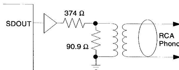
Figure 8. IEC-958 Consumer Interface
