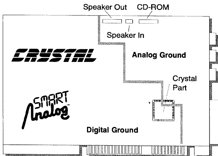
Figure 32. Suggested Add-In Card Layout
