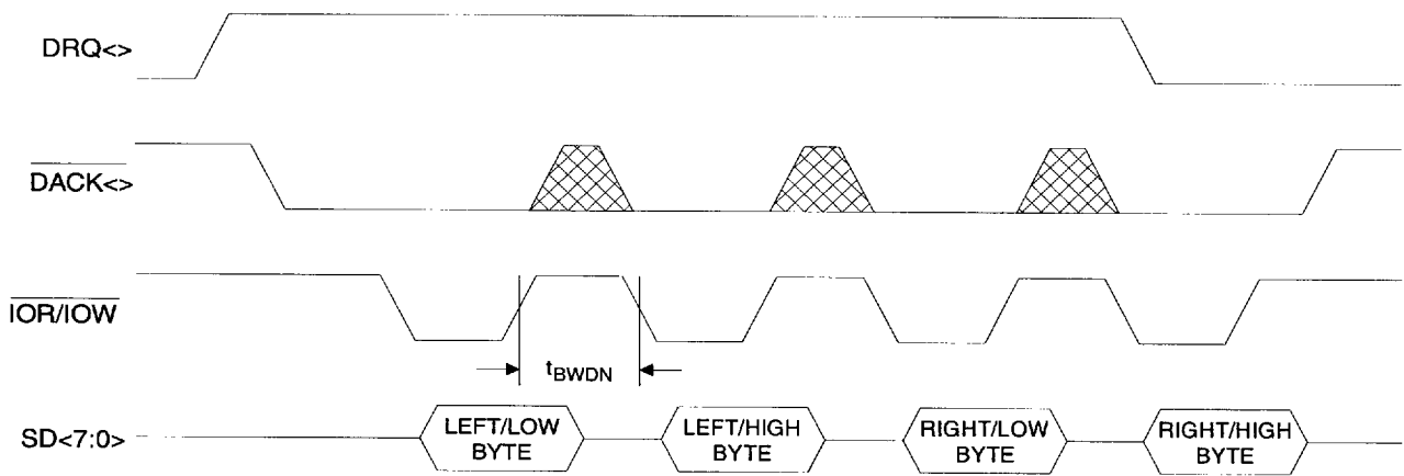
16-Bit Stereo or ADPCM DMA Cycle
