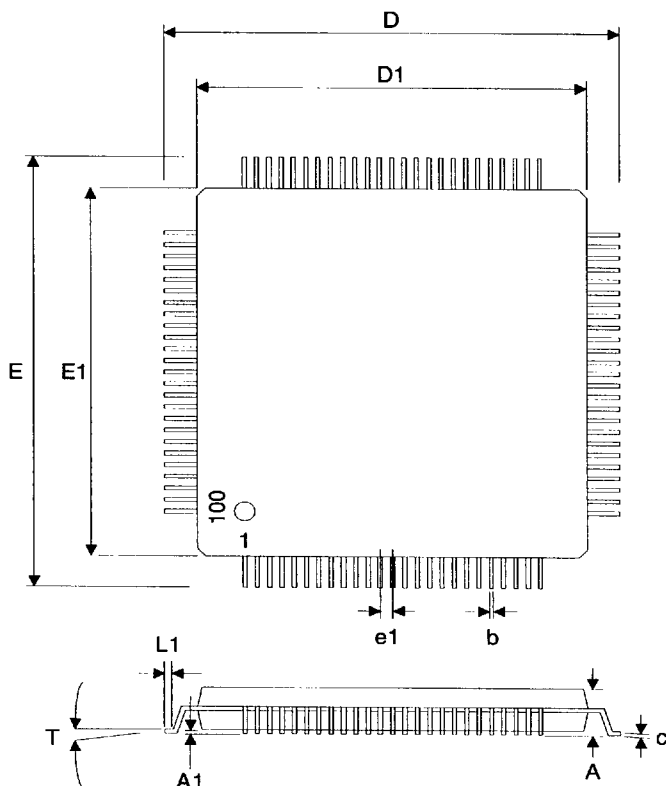
100-pin TQFP - Package Code 'Q'
