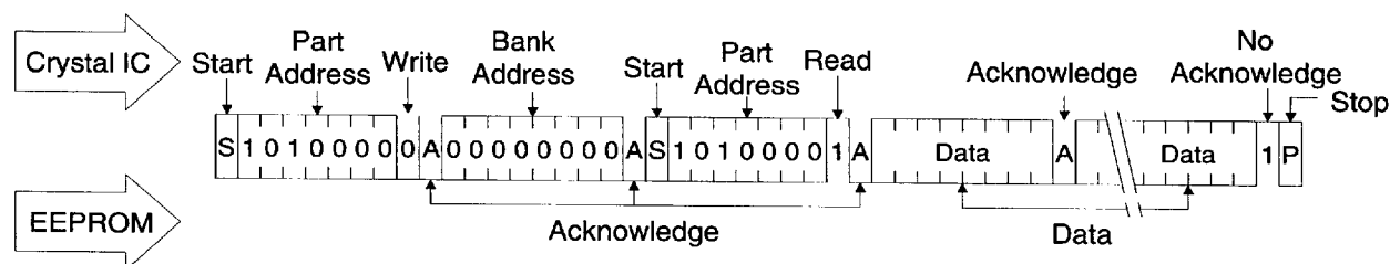
Figure 3. EEPROM Format
