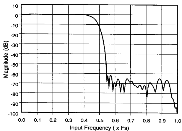
Figure 37. DAC Filter Response
