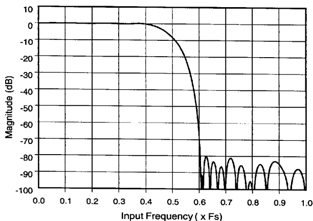
Figure 34. ADC Filter Response
