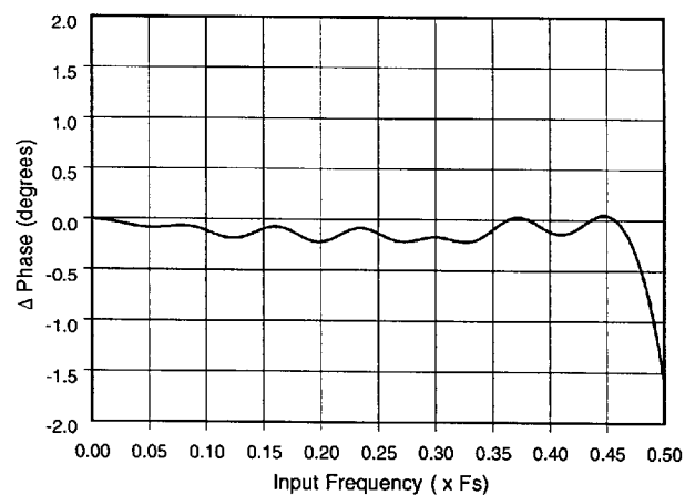
Figure 40. Deviation from Linear Phase
