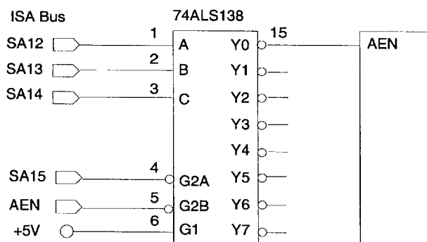
Figure 2. 16-bit Decode Circuit
