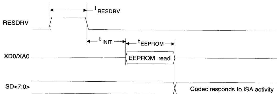
8-Bit Mono DMA Read/Capture Cycle
