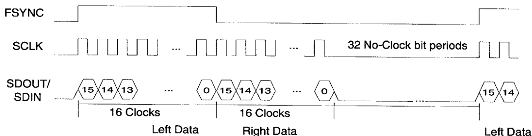
Figure 11. 32-bit Mode (SF1,0 = 10)
