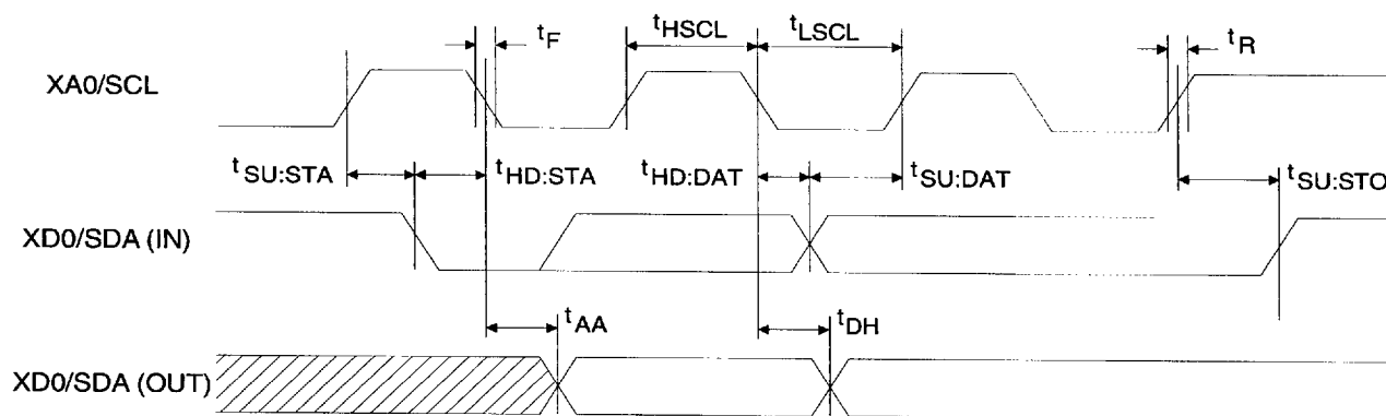
E 2 PROM 2-Wire Interface Timing
