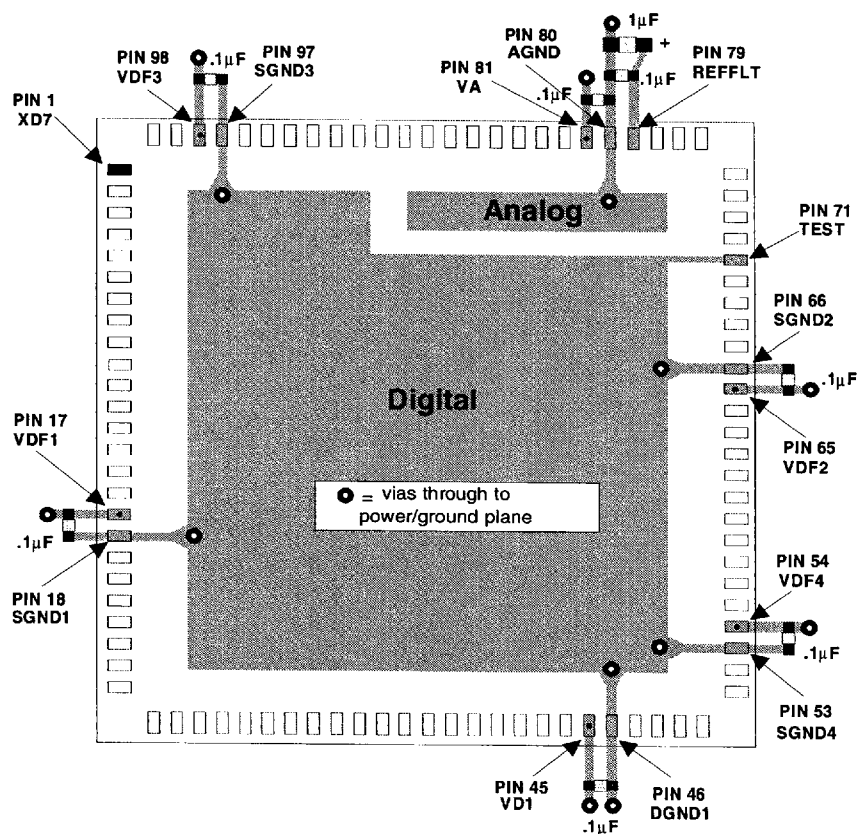
Figure 33. Recommended Decoupling Capacitor Positions
