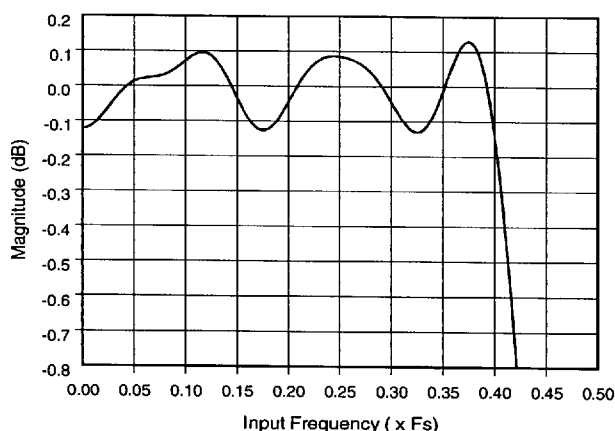
Figure 35. ADC Passband Ripple
