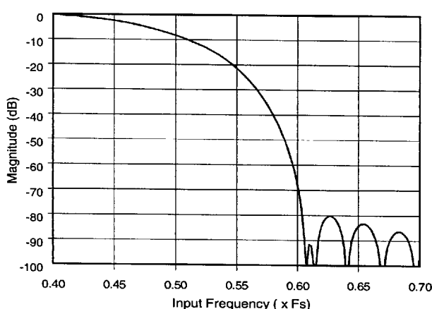
Figure 36. ADC Transition Band
