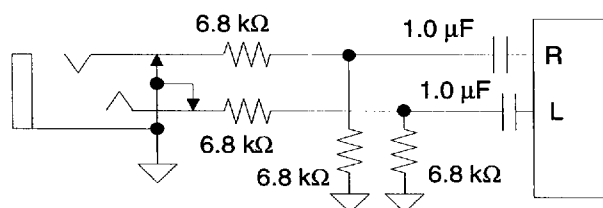
Figure 26. Line Inputs
