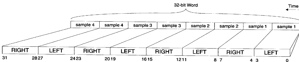
Figure 19. 4-bit Stereo, ADPCM Audio Data
