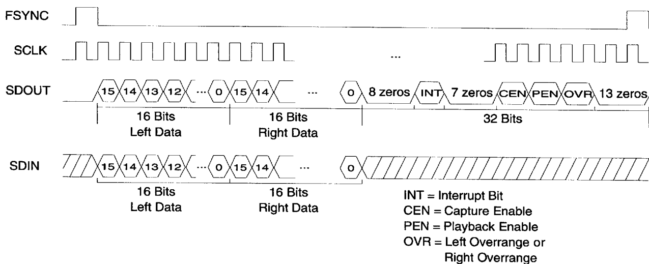
Figure 9. 64-bit Enhanced Mode (SF1,0 = 00)
