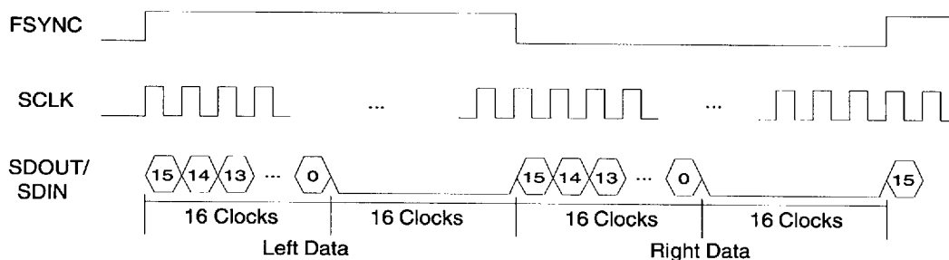
Figure 10. 64-bit Mode (SF1,0 = 01)
