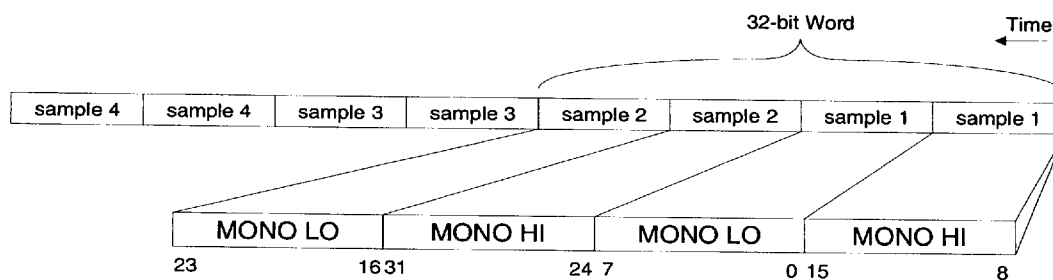
Figure 20. 16-bit Mono, Signed Big Endian Audio Data
