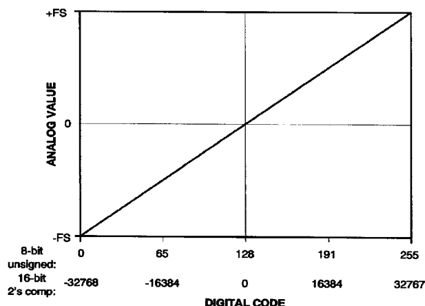
Figure 22. Linear Transfer Functions
