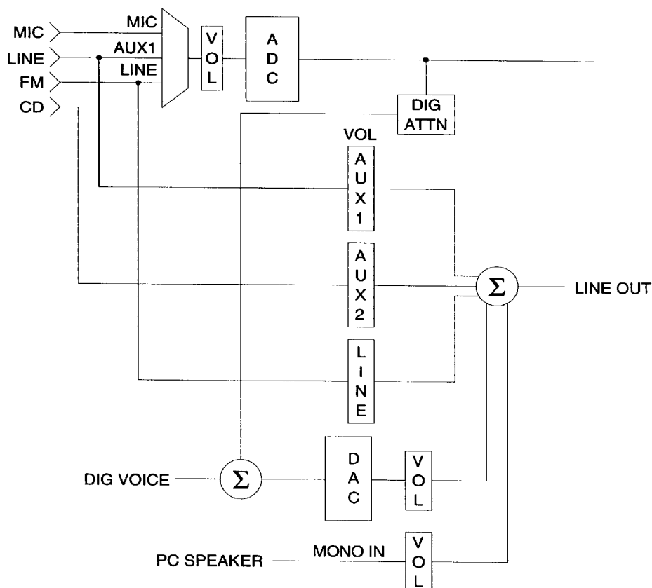
Figure 5. SBPro Mixer Mapping
