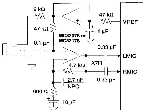
Figure 28. Left or Mono Microphone Input
