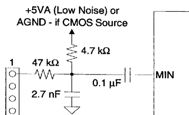
Figure 29. Mono Input
