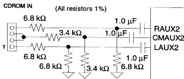
Figure 27. Differential CDROM In
