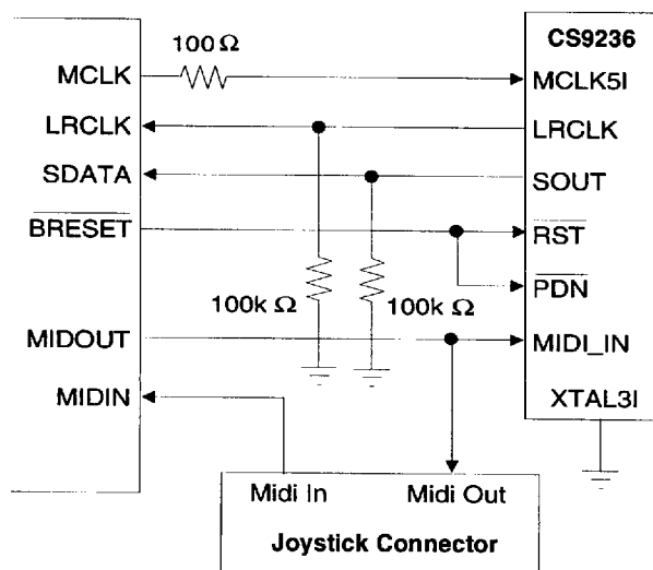
Figure 13. CS9236 Wavetable Serial Port Interface
