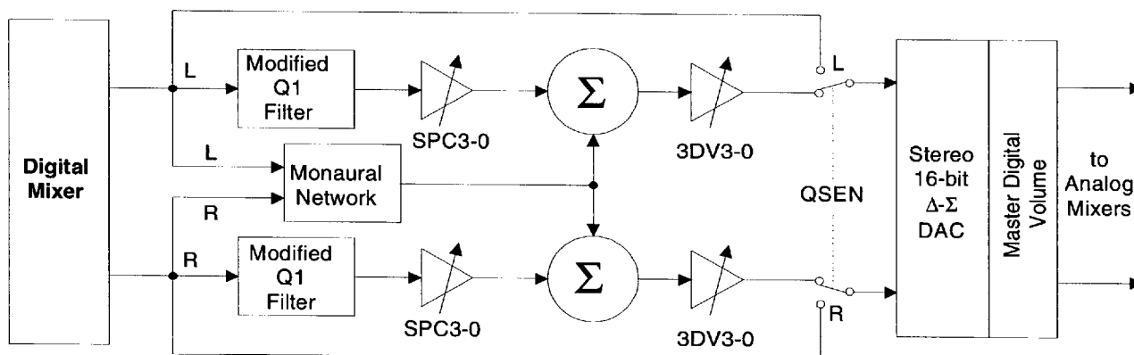
Figure 7. QXpander Block Diagram
