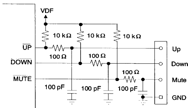
Figure 24. Volume Control Circuit
