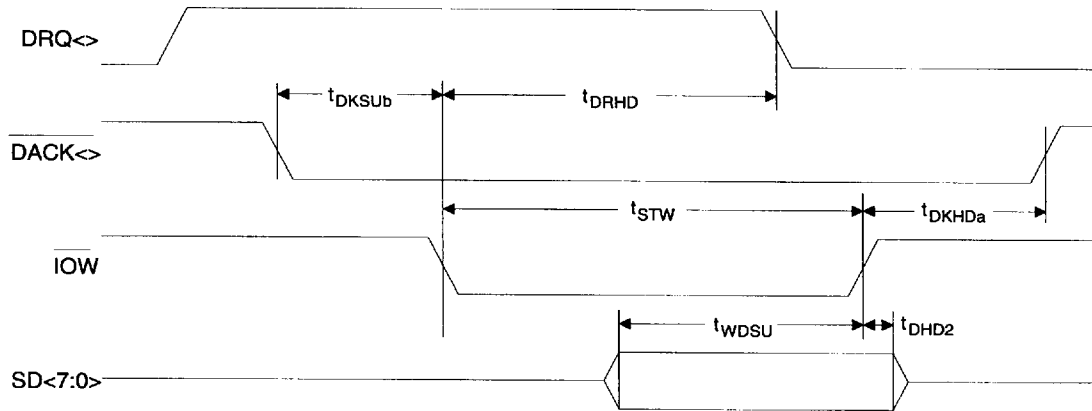
8-Bit Mono DMA Write/Playback Cycle
