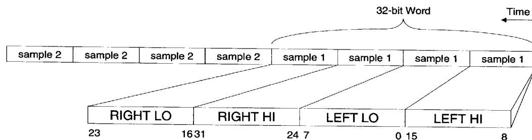
Figure 21. 16-bit Stereo, Signed Big Endian Audio Data
