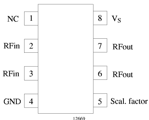
Figure 2. Pinning
