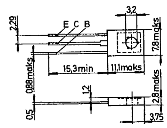
TO-126
