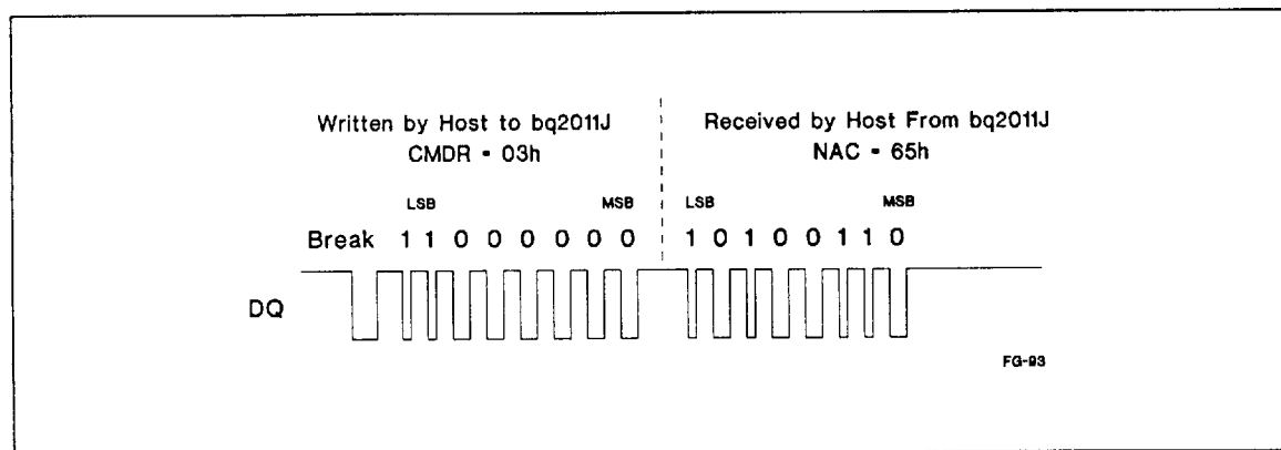
Figure 3. Typical Communication With the bq2011J
