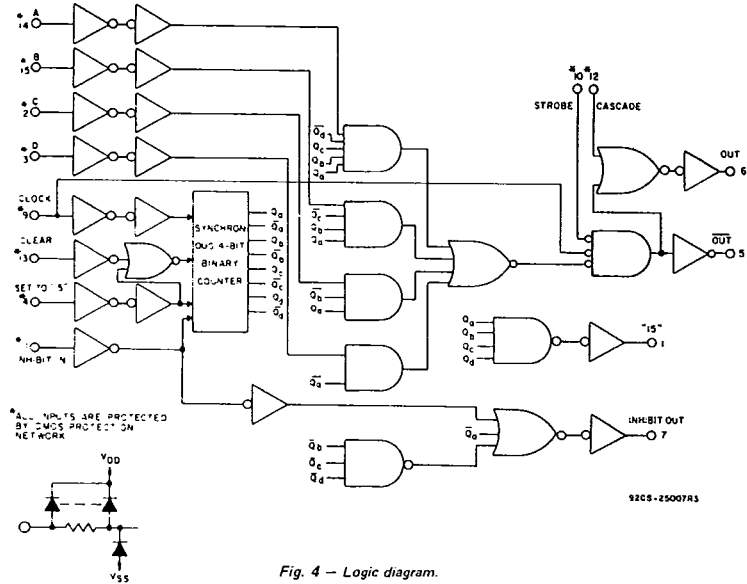
Fig. 4 — Logic diagram.
