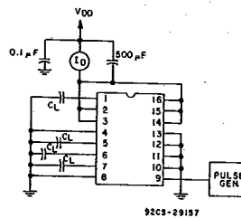
Fig. 9 — Dynamic power dissipation test circuit.
