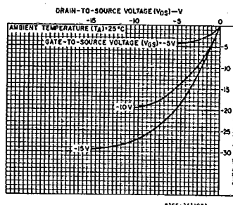
Fig. 3 - Typical output high (source) current characteristics.
