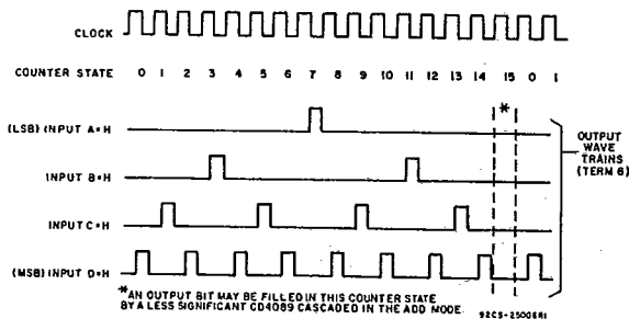
Fig. 15 – Timing diagram.
