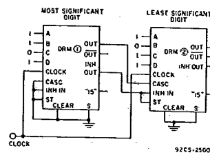
Fig. 13 – Two CD4089B's cascaded in the "Add" mode with a preset number
