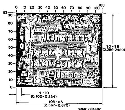
Dimensions and Pad Layout for CD4089BH
