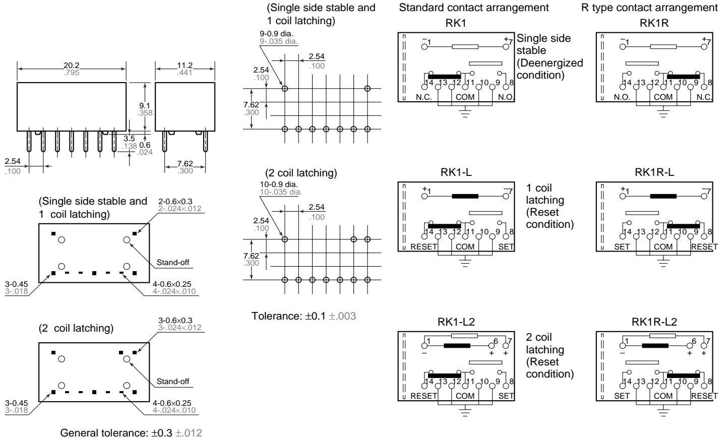
PC board pattern (Copper-side view)
