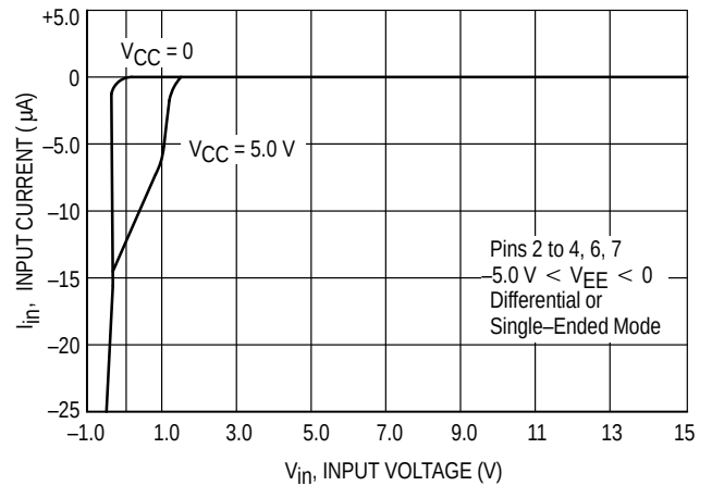
Figure 9. Input Current versus Input Voltage
