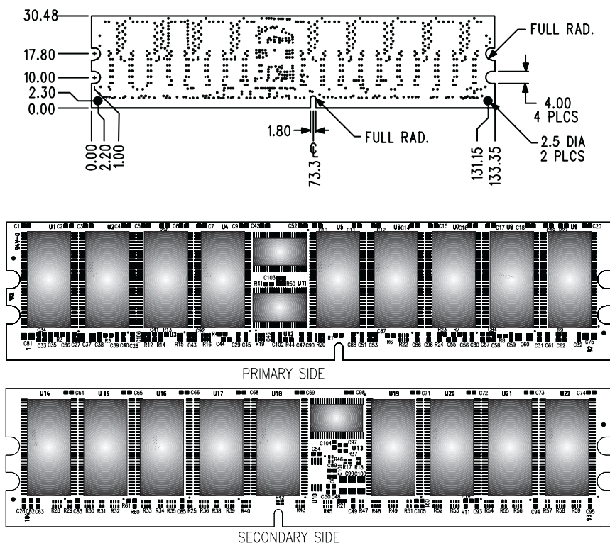
Figure 1: KVR266X72RC25L/512 184-Pin DIMM
