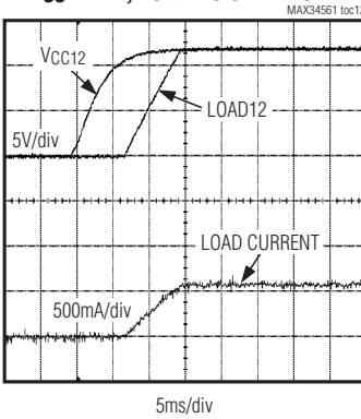
TURN-ON WAVEFORMS V_{CC} = 12\text{V} , 20\Omega RESISTIVE LOAD
