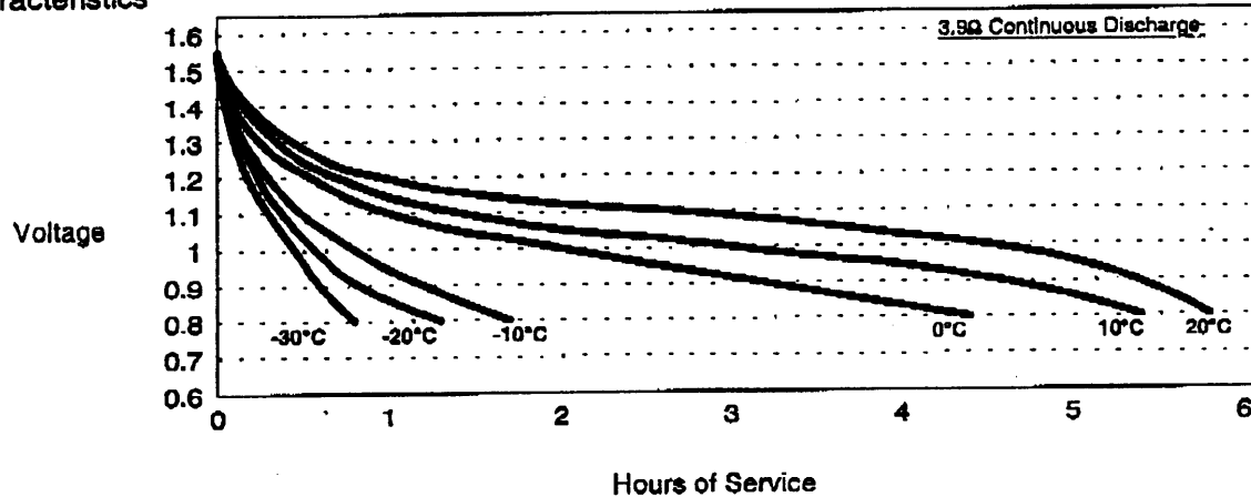
Typical Discharge Characteristics
