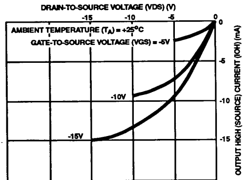
FIGURE 12. MINIMUM OUTPUT HIGH (SOURCE) CURRENT CHARACTERISTICS
