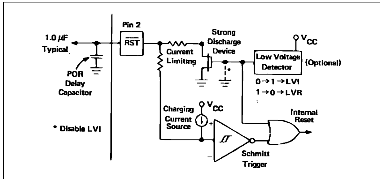
Figure 14 : RESET Configuration.
