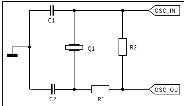
Figure 11: Oscillator Circuitry
