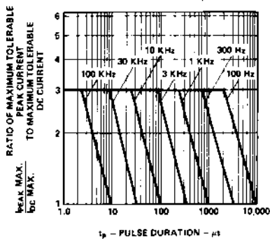
Figure 15. Maximum Tolerable Peak Current vs. Pulse Duration ( I_{\text{DC MAX}} as per MAX Ratings).
