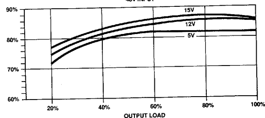
TYPICAL EFFICIENCY VS. OUTPUT LOAD 48V INPUT
