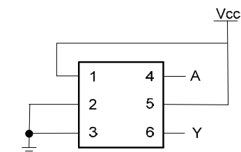
Configuration 6 Buffer
