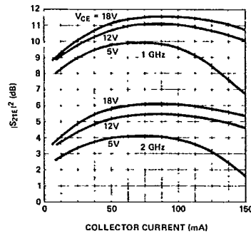
Figure 8. Typical S_{21}^2 vs. Collector Current at 1 and 2 GHz, for the HXTR-5101.
