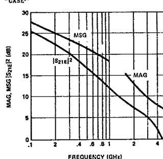
Figure 2. Typical MAG, Maximum Stable Gain (MSG), and |S 21 | 2 vs. Frequency (V CE = 18 V, I C = 110 mA), for the HXTR-5102.
