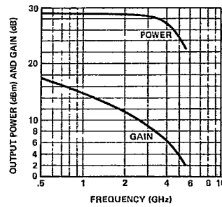
Figure 9. Typical P_{1dB} and Associated 1 dB Compressed Gain vs. Frequency ( V_{CE} = 18 V, I_C = 110 mA), for the HXTR-5102.
