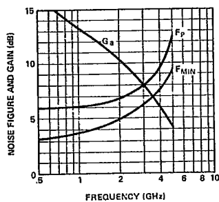
Figure 16. Typical Noise Figure ( NF_{MIN} ) and Associated Gain ( G_A ) when Tuned for Minimum Noise vs. Frequency V_{CE} = 18 V, I_C = 25 mA, Typical Noise Figure ( F_P ) when Tuned for Max P1dB ( V_{CE} = 18 V, I_C = 110 mA), for the HXTR-5102.
