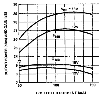
Figure 6. Typical P 1dB and Associated 1 dB Compressed Gain vs. Collector Current (V CE = 12 V and 18 V at 2 GHz), for the HXTR-5104.
