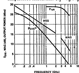
Figure 1. Typical |S 21 | 2 , MAG and P 1dB Linear Power vs. Frequency (V CE = 18 V, I C = 110 mA), for the HXTR-5002.
