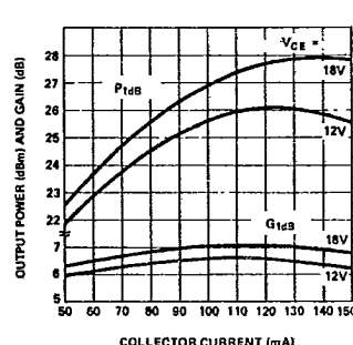
Figure 5. Typical P 1dB and Associated 1 dB Compressed Gain vs. Collector Current (V CE = 12 V and 18 V at 4 GHz), for the HXTR-5102.
