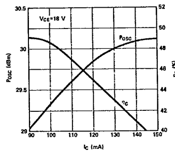
Figure 18. Typical Oscillator Power and Efficiency vs. Collector Current at f = 2 GHz, for the HXTR-4103.
