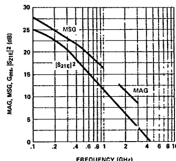
Figure 3. Typical MAG, Maximum Stable Gain (MSG), and |S 21 | 2 vs. Frequency (V CE = 18 V, I C = 110 mA), for the HXTR-5104.
